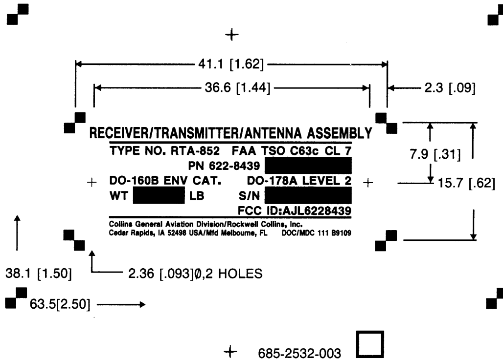
Figure 12. RTA-8XX Equipment Nameplate Drawing, Collins Part Number 685-2532-003
