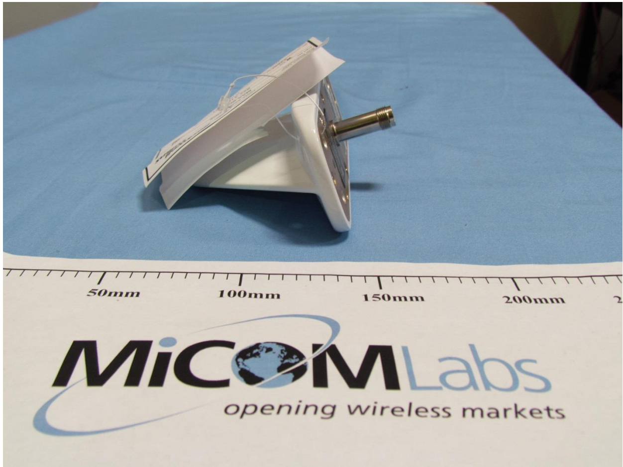
MAA-6000 Side 3 View
