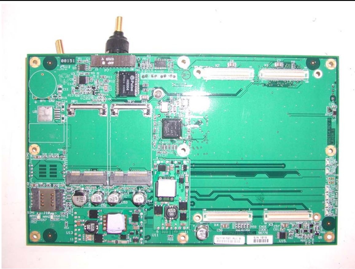
Figure I-5. UMTS-2100 Carrier Board (ETLX and Modem removed)
