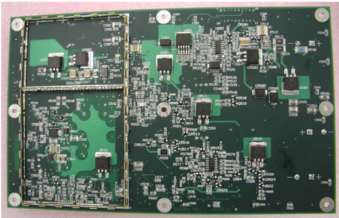
Figure I-13. UMTS-2100 Power Supply Board (bottom) (without shield)
