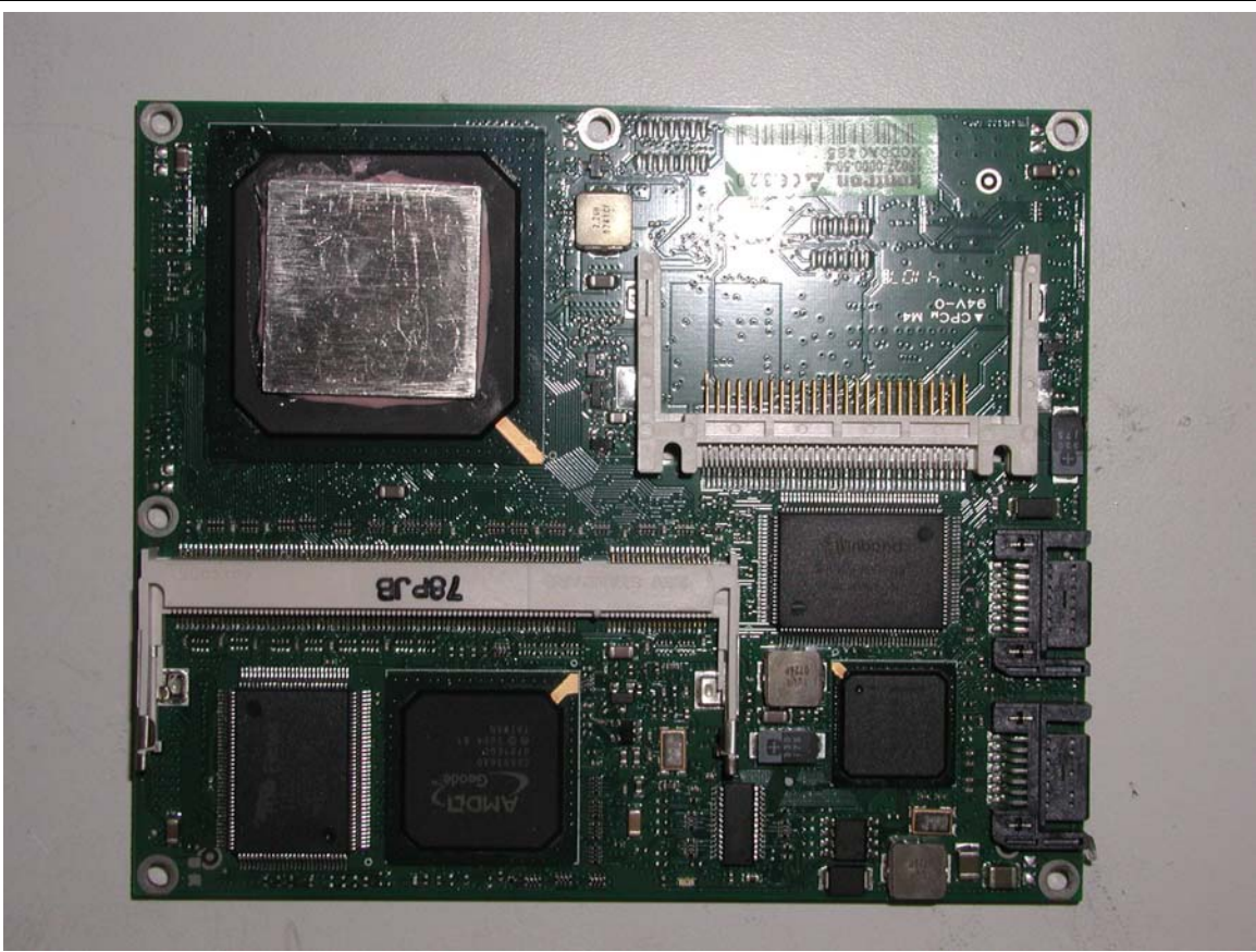
Figure I-9. UMTS-2100 ETLX Processor Board(RAM and CF memory removed)
