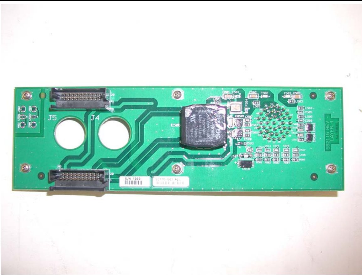
Figure I-11. UMTS-2100 I/O Board (bottom)
