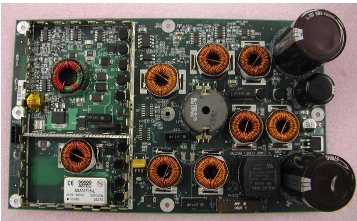
Figure I-12. UMTS-2100 Power Supply Board (top) (without shield)
