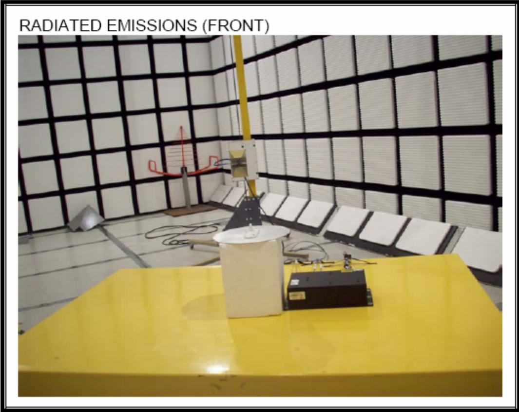
Figure G-1. UMTS-2100 Radiated Emissions (Front)
