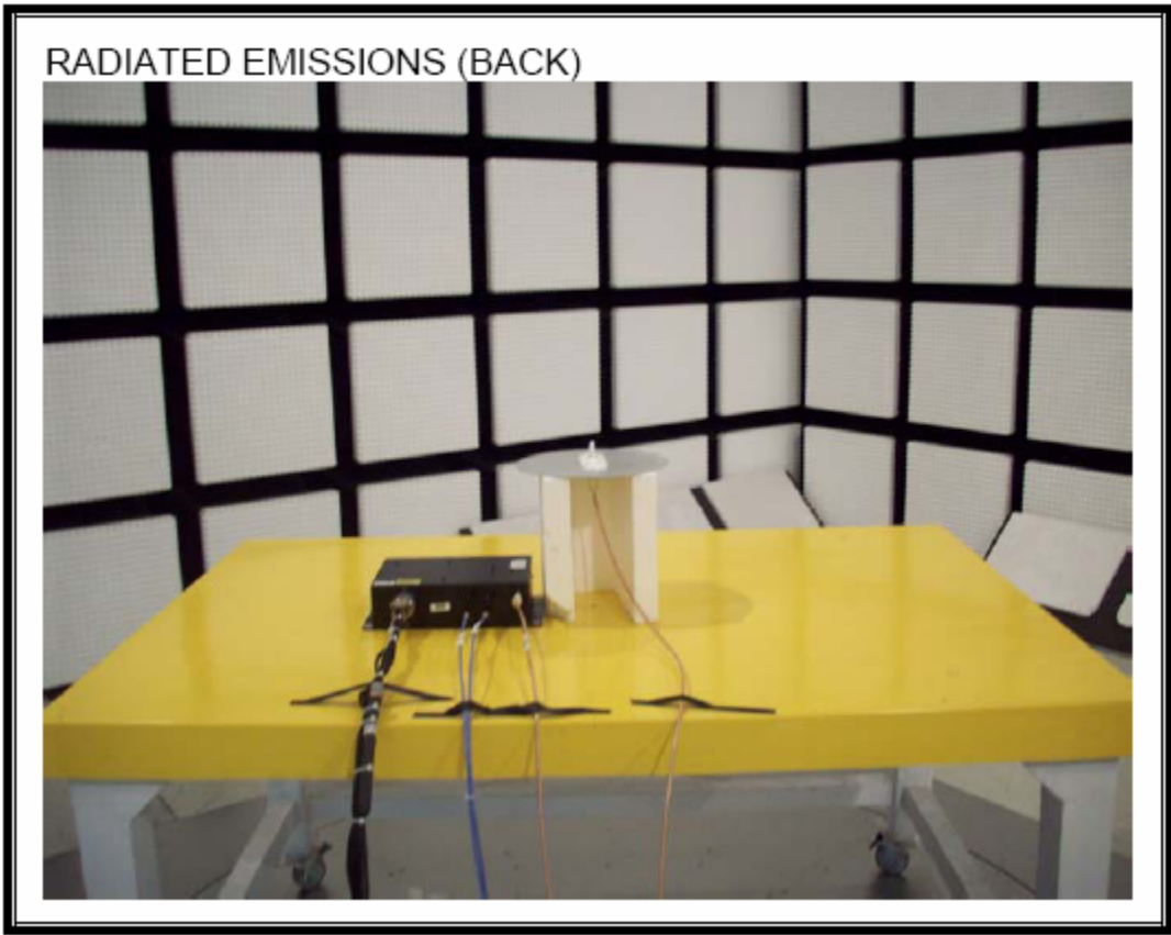
Figure G-2. UMS-2100 Radiated Emissions (Back)
