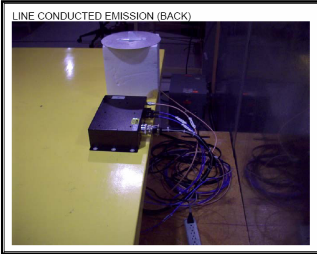
Figure G-4. UMS-2100 AC Mains Line Conducted Emission (Back)
