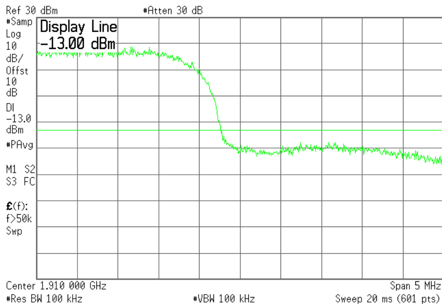
Plot 7.4.12) WCDMA; PCS high channel, above 1910 MHz
