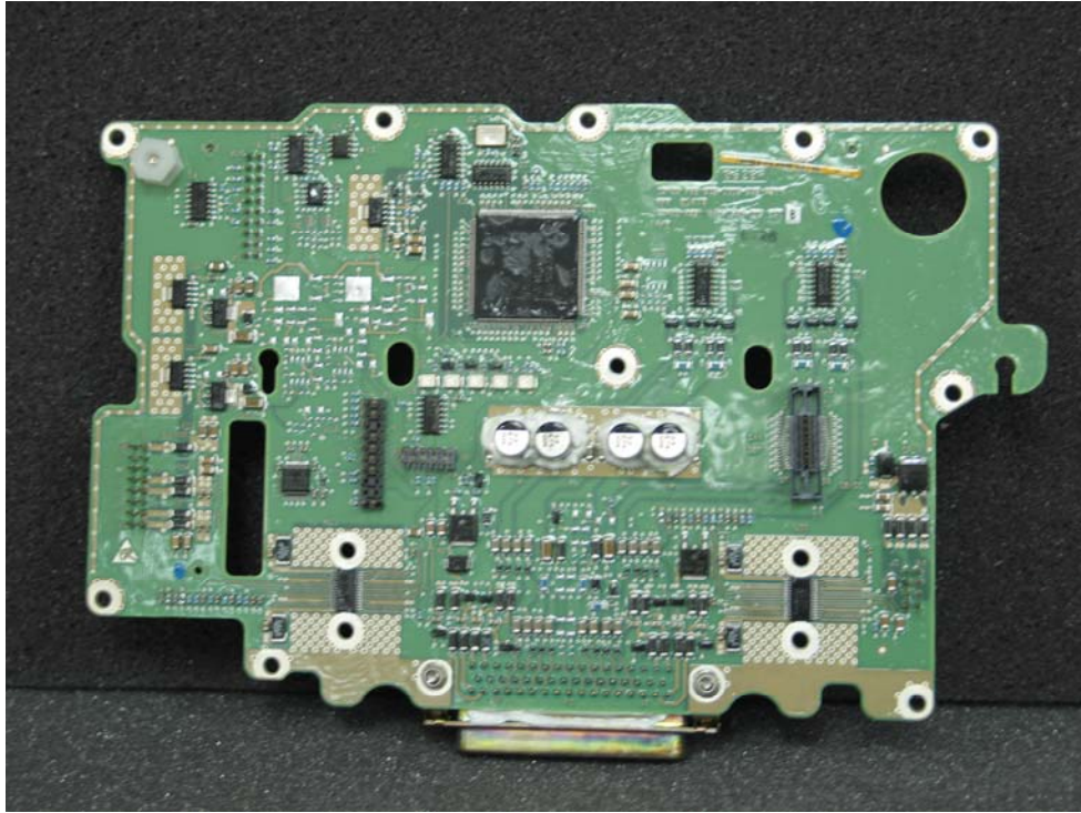
Figure I-8. Antenna Drive card (top)
