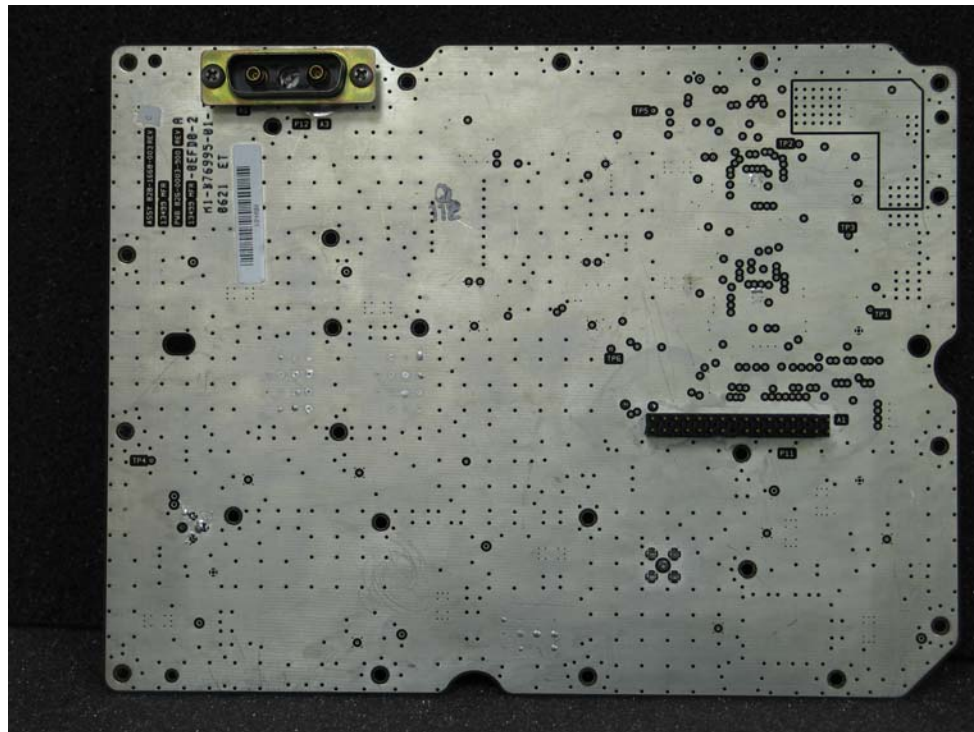
Figure I-5. DDS Source card (bottom)
