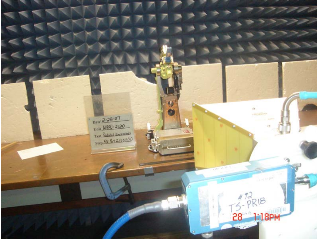
Figure G-6. Radiated Emission 1 GHz – 18 GHz
