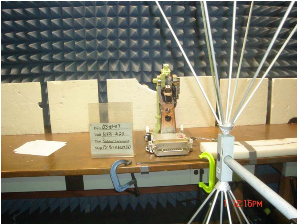
Figure G-4. Radiated Emission 25 MHz – 200 MHz
