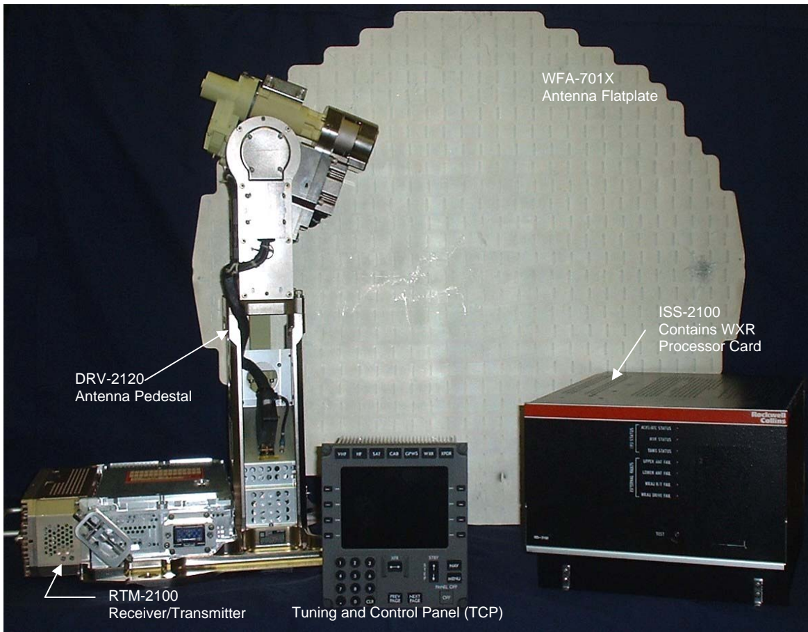
Figure C-1. Weather Radar System Components
