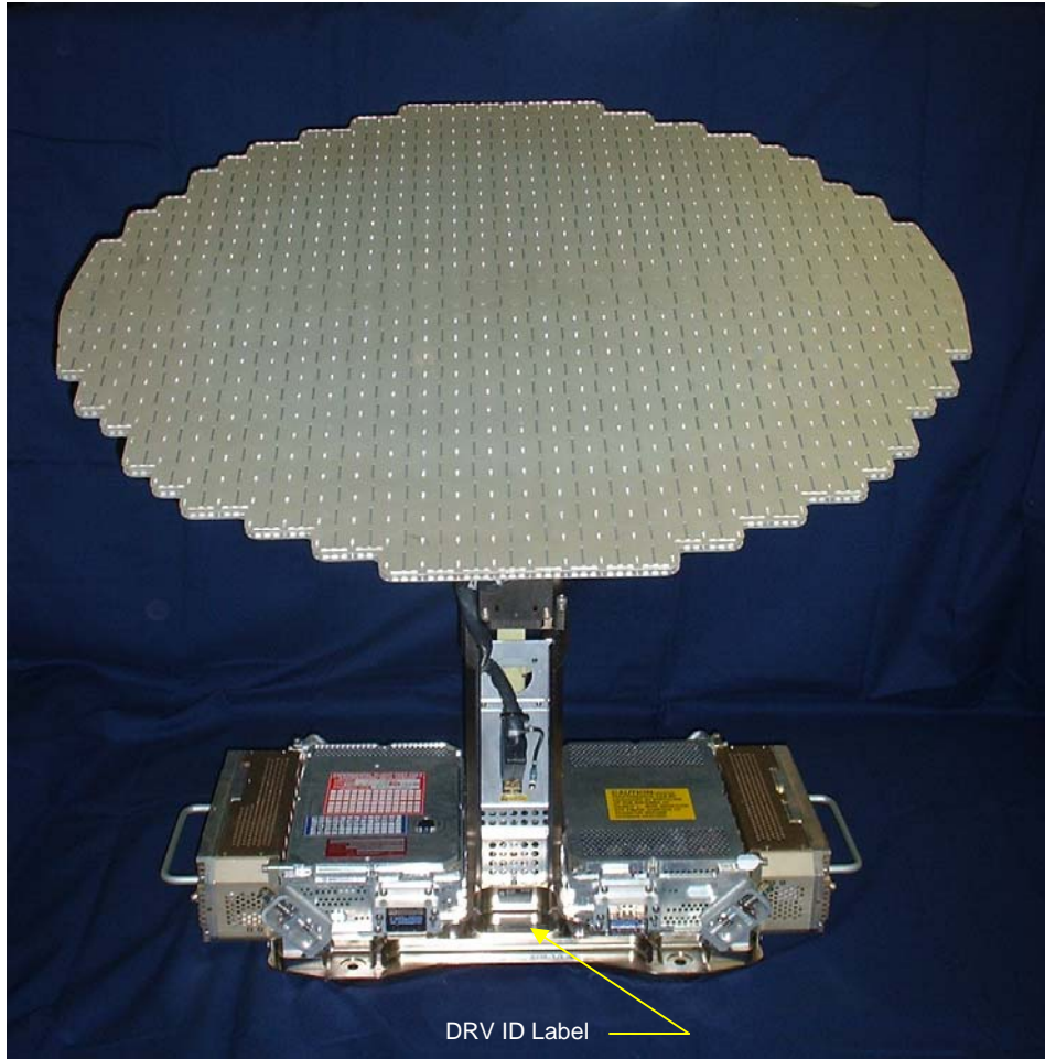
Figure C-3. WRAU-2120 (opp. side)
