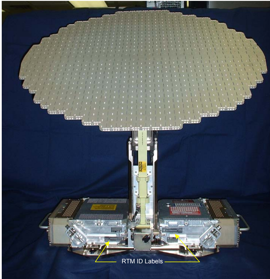
Figure A-3. WRAU-2120 showing RTM-2100 ID Label locations
