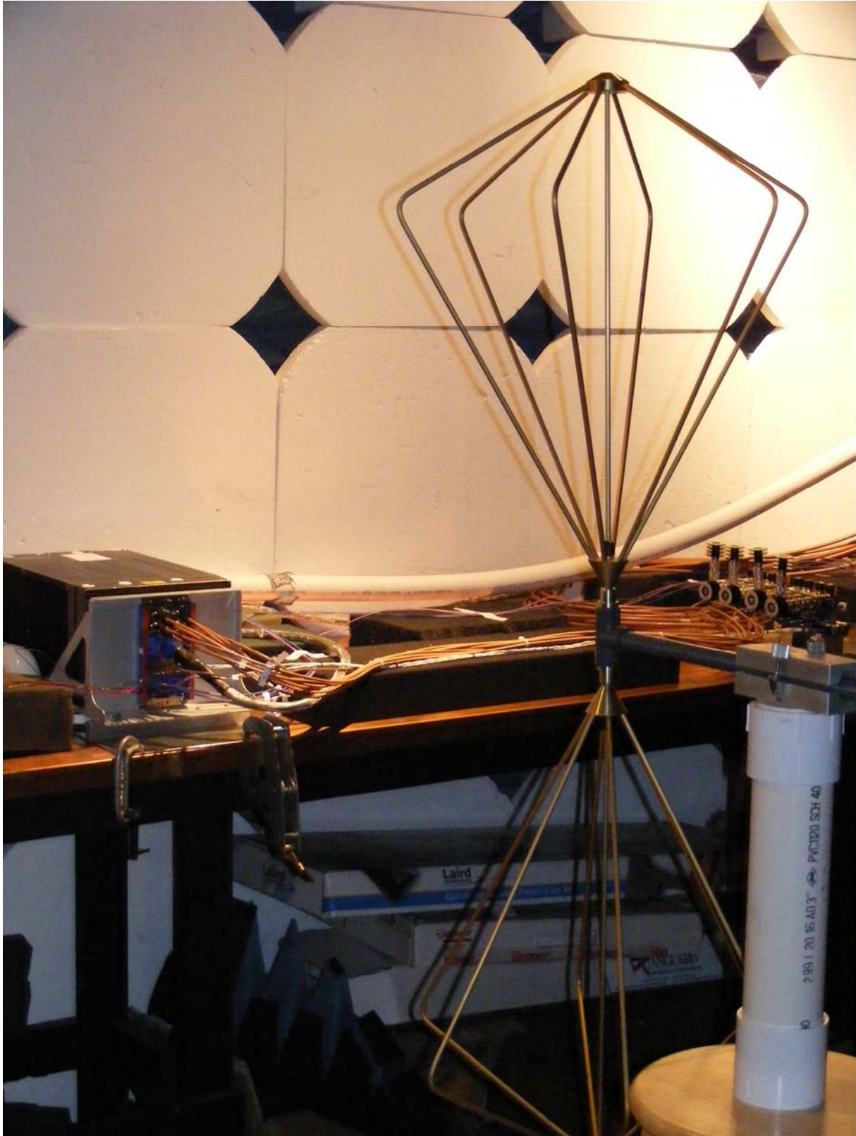
Figure 3 – Radiated Emissions Test. Biconical Antenna in Vertical Polarization
