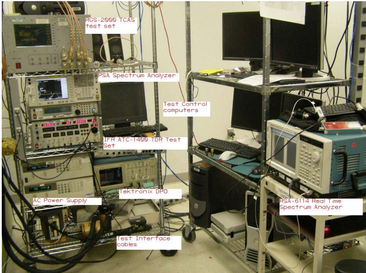
Figure 1 – Computer Aided Test Set
