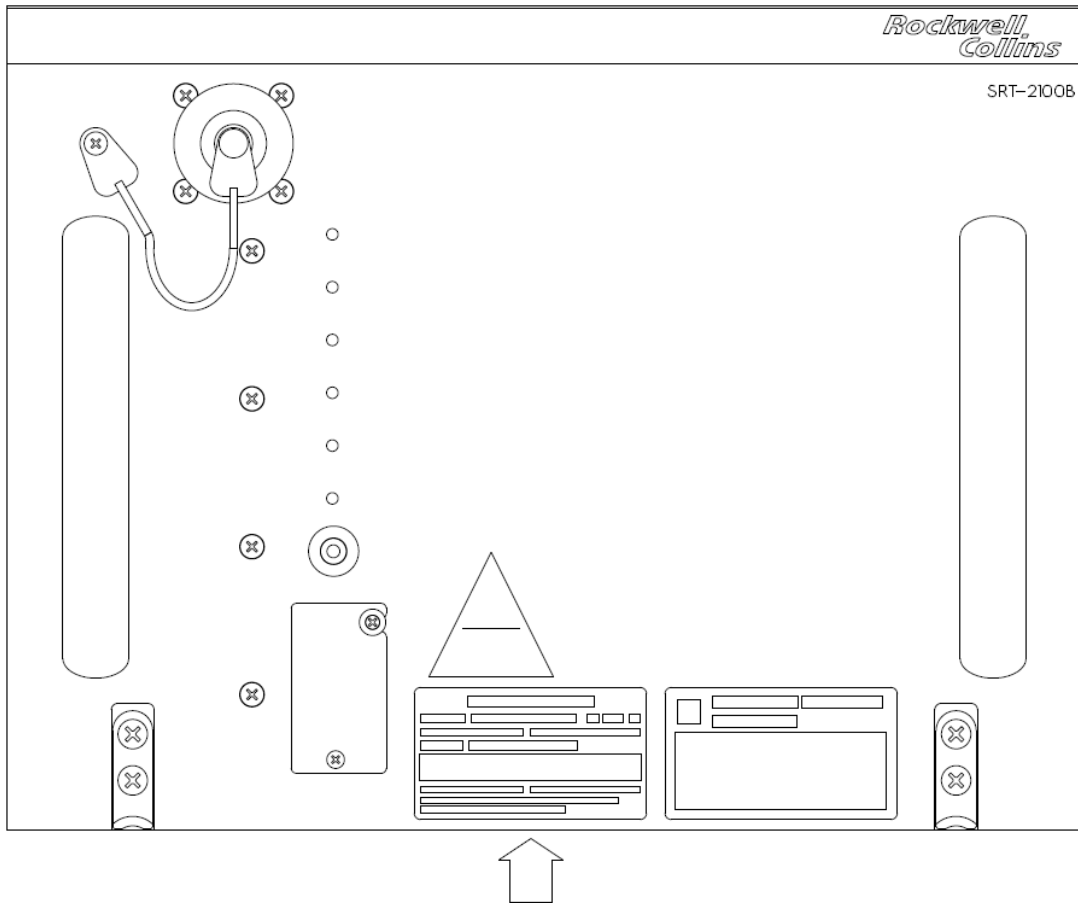
Figure 2 SRT-2100B Front Panel showing nameplate location
