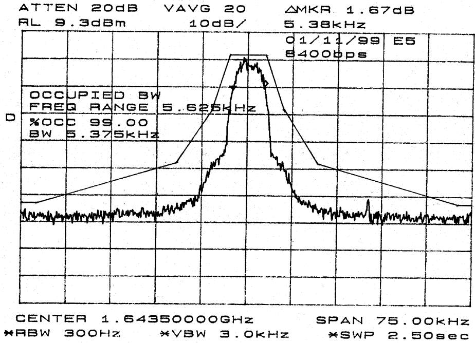
Figure 9.6.2.3 Bandwidth Occupancy Test – Power 25 Watts
