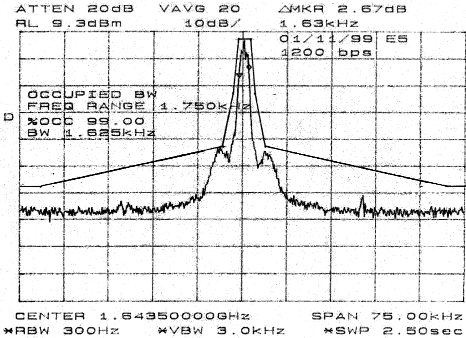
Figure 9.6.2.2 Bandwidth Occupancy Test – Power 25 Watts
