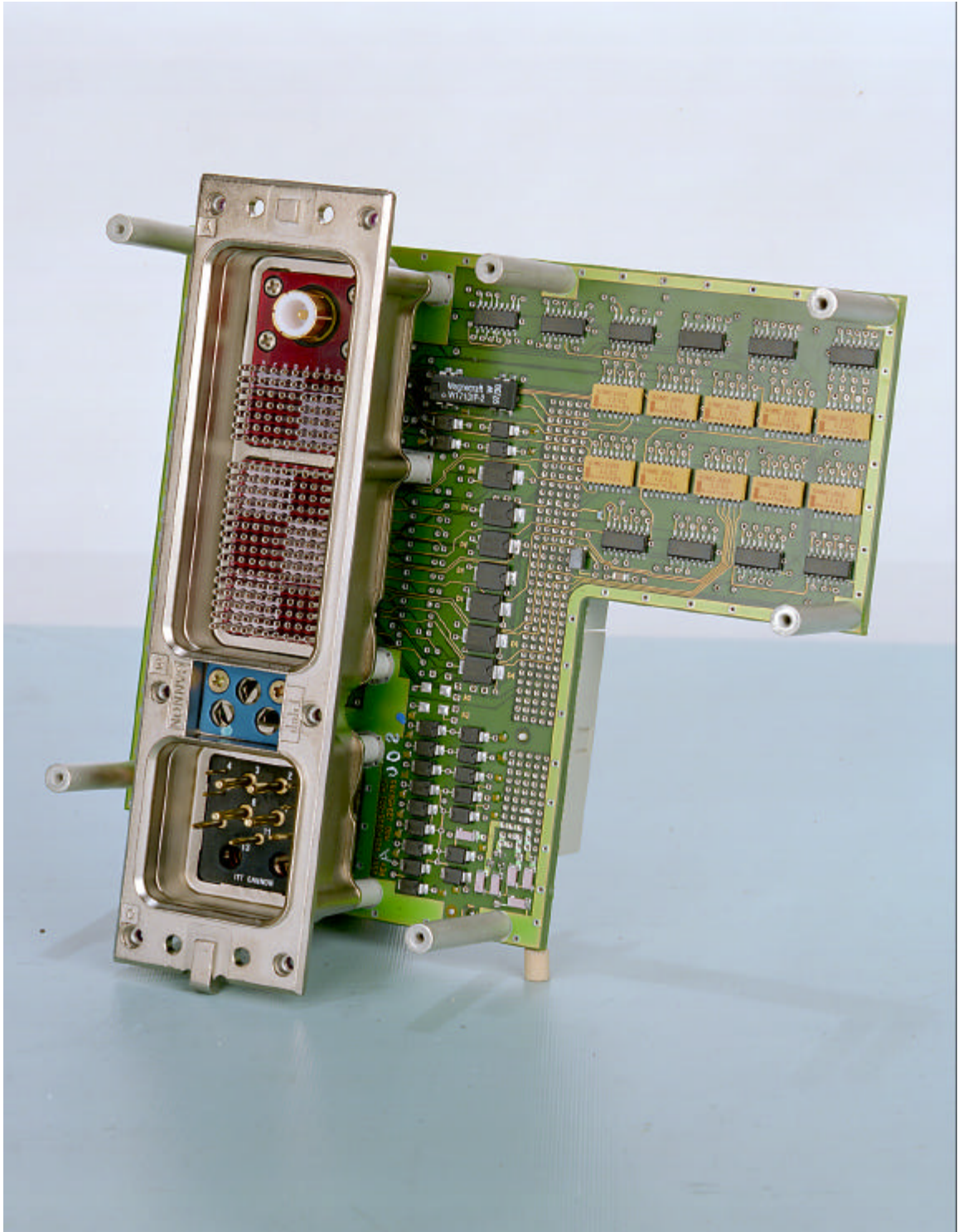
Figure 8-8 Rear Interconnect Card Assembly
