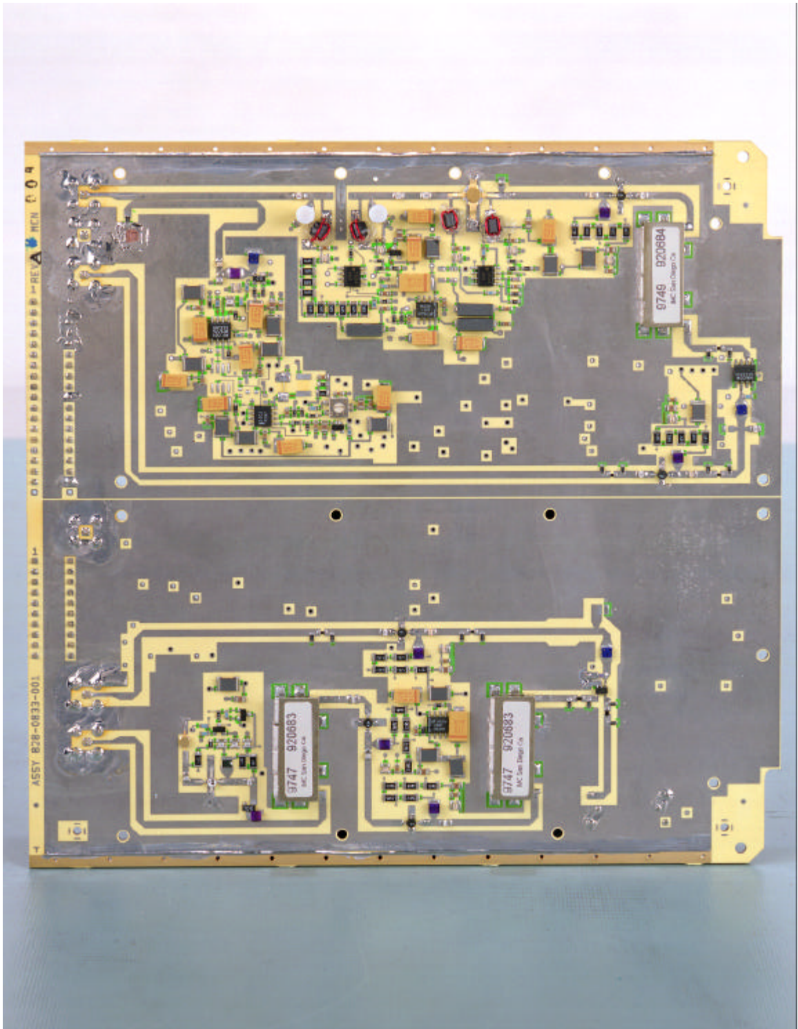
Figure 8-6 Up/Down Converter Card Assembly (Top View)
