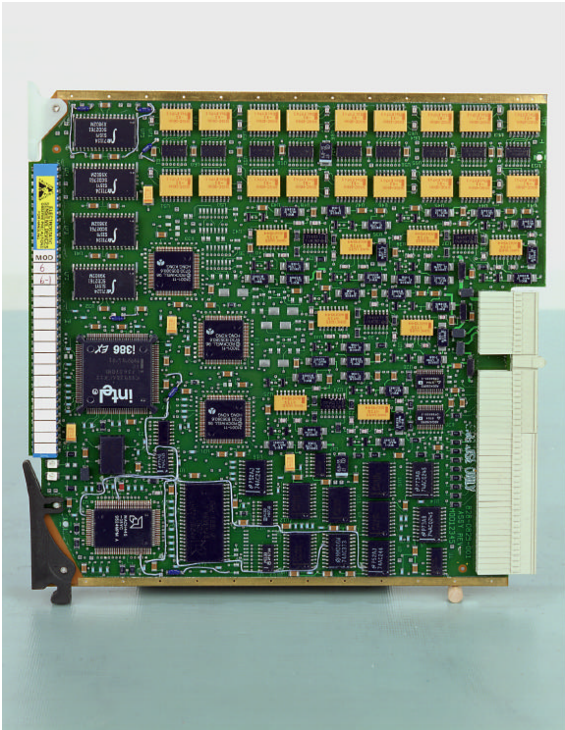
Figure 8-11 429 I/O Card Assembly
