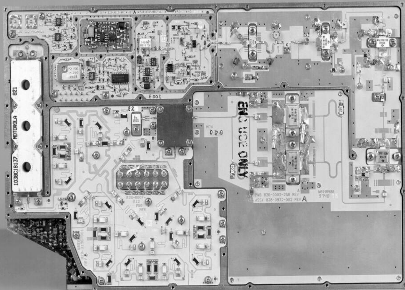
Transmitter Module
