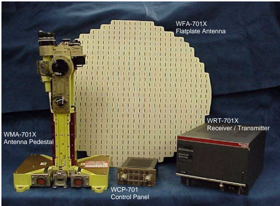
Figure C-1. WXR-701X Family
