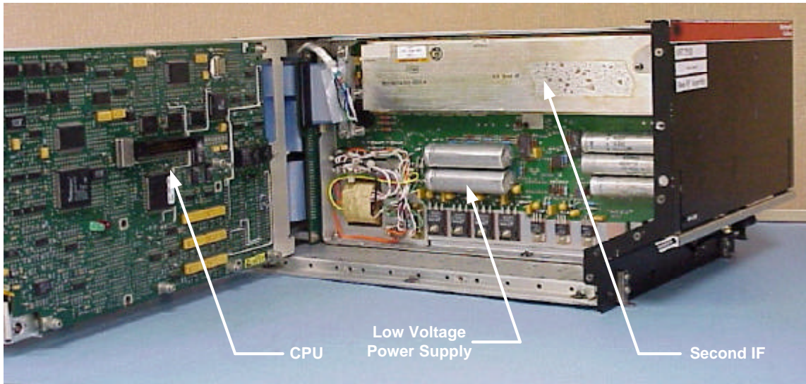
Figure I-2. Chassis Left Open
