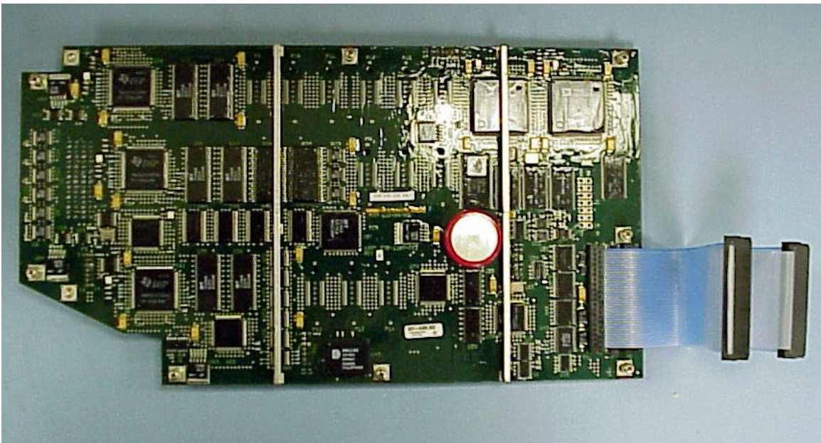
Figure I-17. DSP Front
