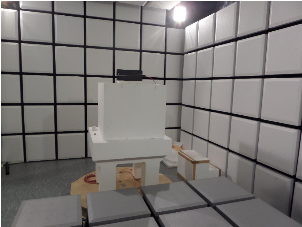
Test in anechoic room
