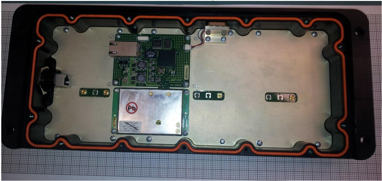
PSR500 without housing and cables:
