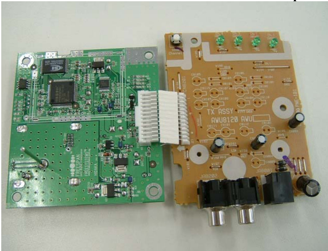
Back Side
