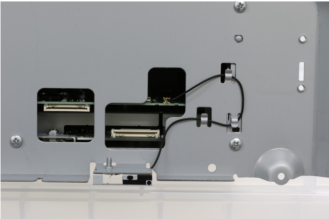
Antenna position
