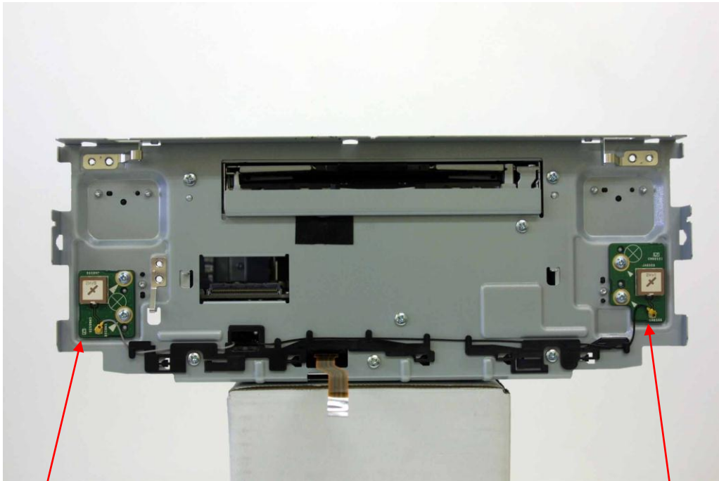
WLAN Antenna
