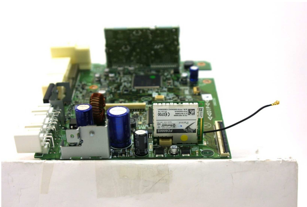
Bluetooth Board Position
