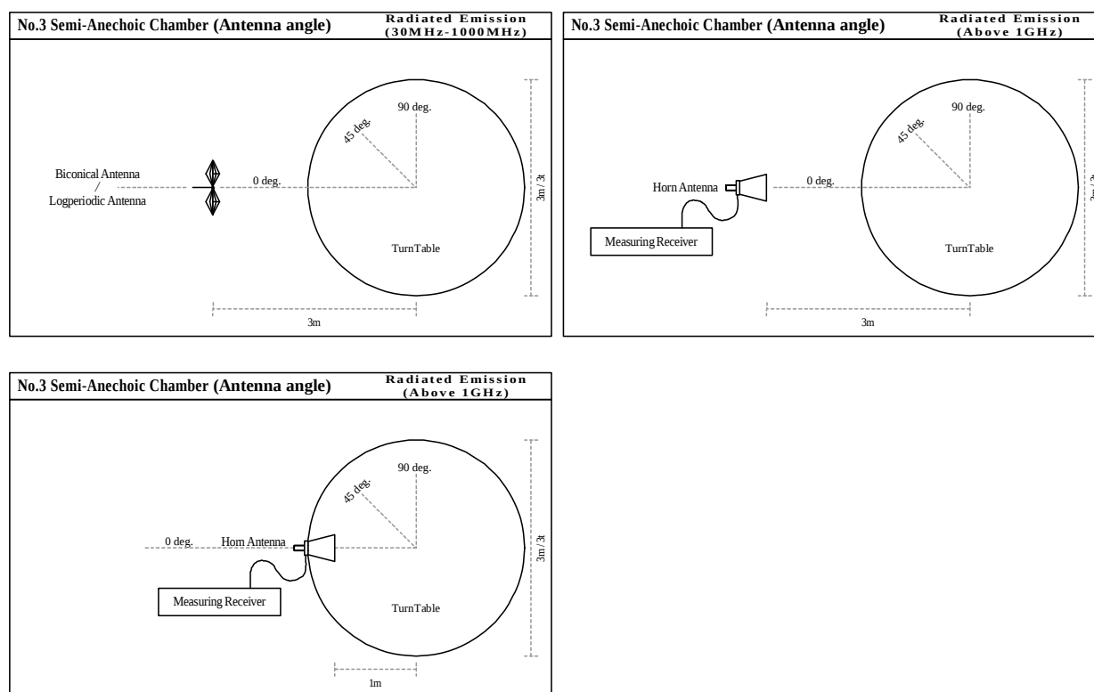
Figure 1. Antenna angle
