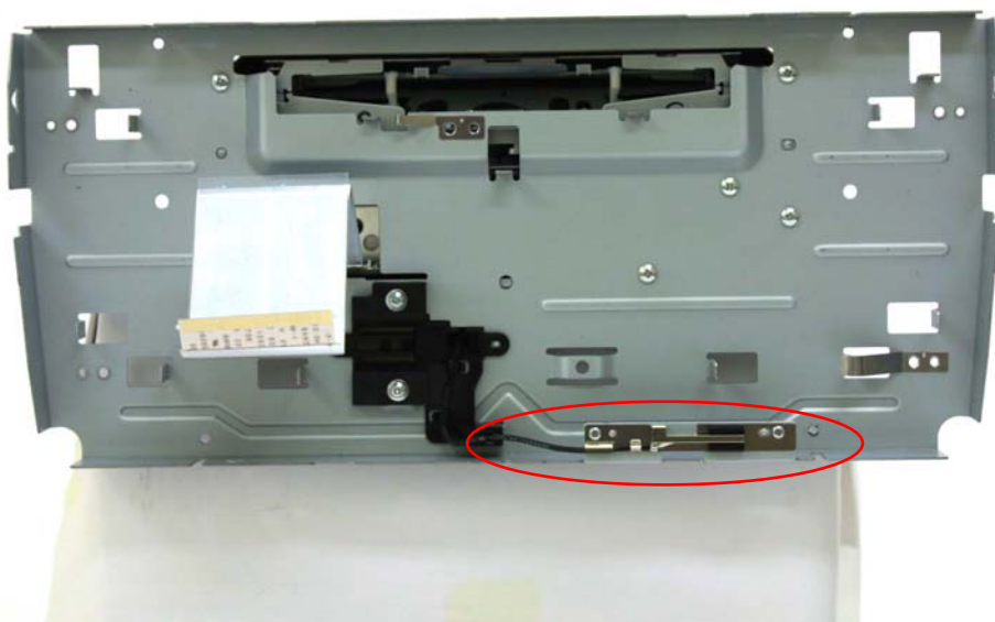
Antenna Position
