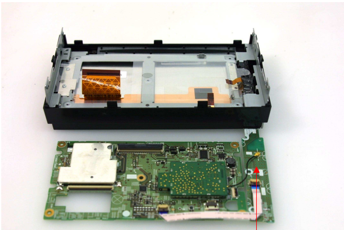
BT Board and Antenna Location
