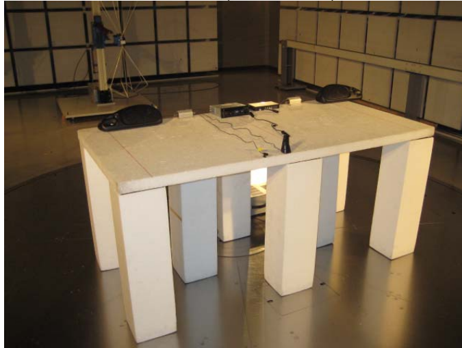
Front view (1-26GHz)
