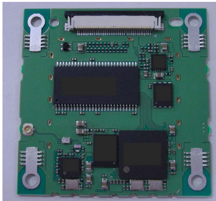
BT Board Side A without Shield
