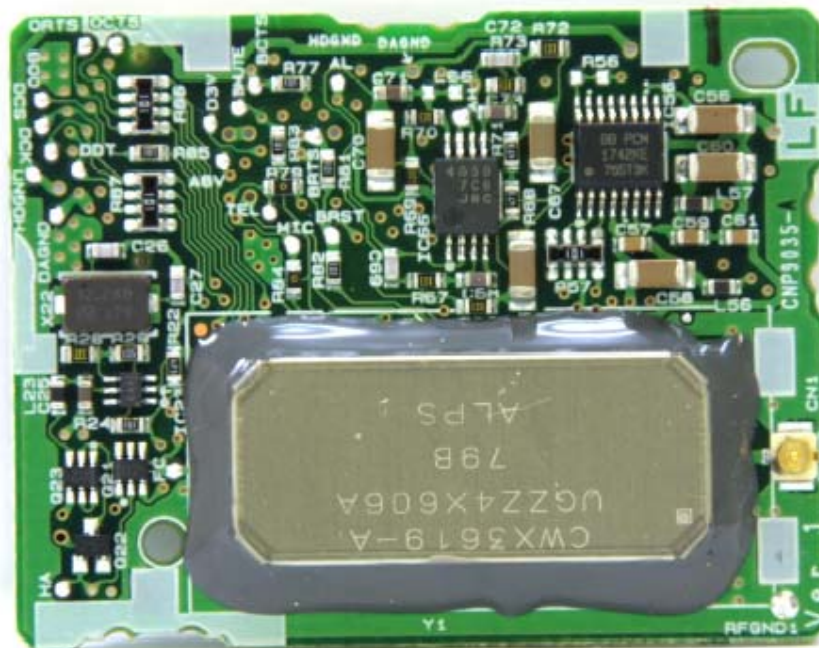
Top View of Blue tooth Module
