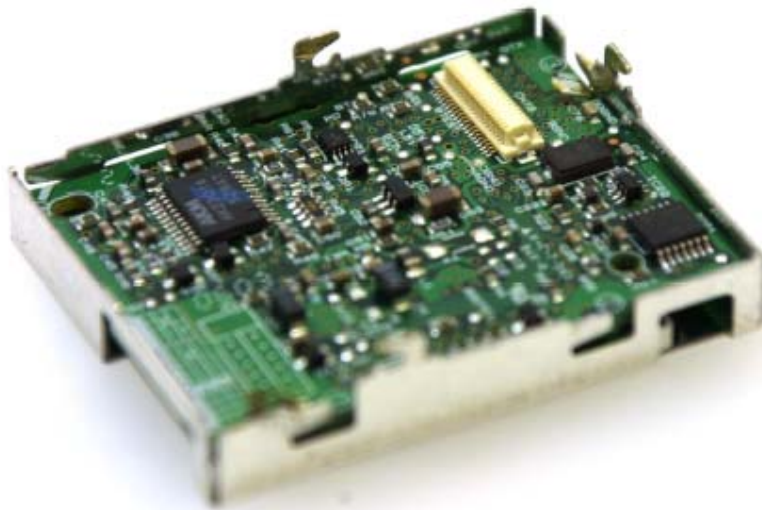
BT Board with Shield Cover(Bottom)
