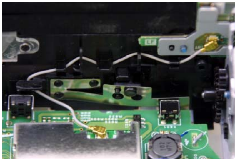
Antenna Location
