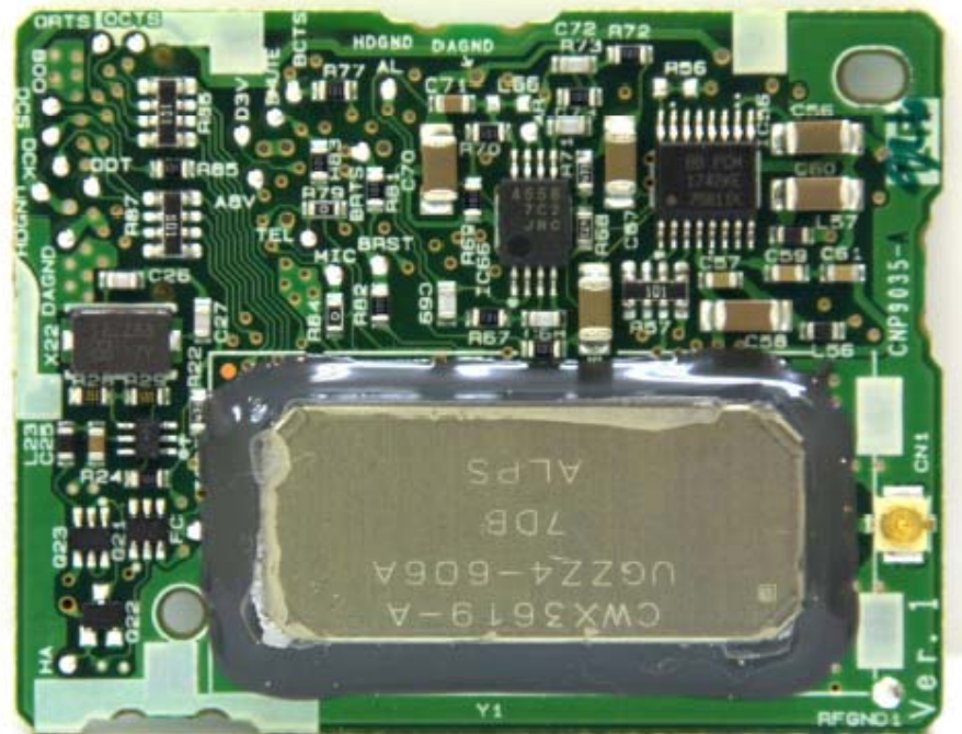
Top View of Bluetooth Board
