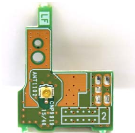
Antenna(Back)
