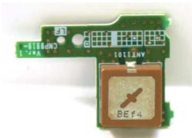
Antenna (front)
