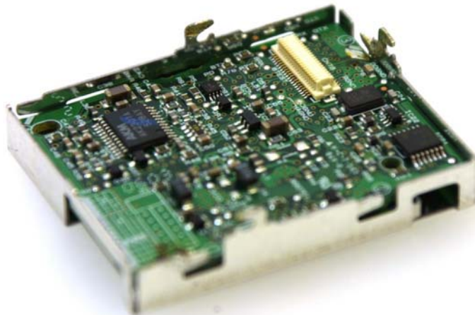
Bluetooth Unit Side B with Shield
