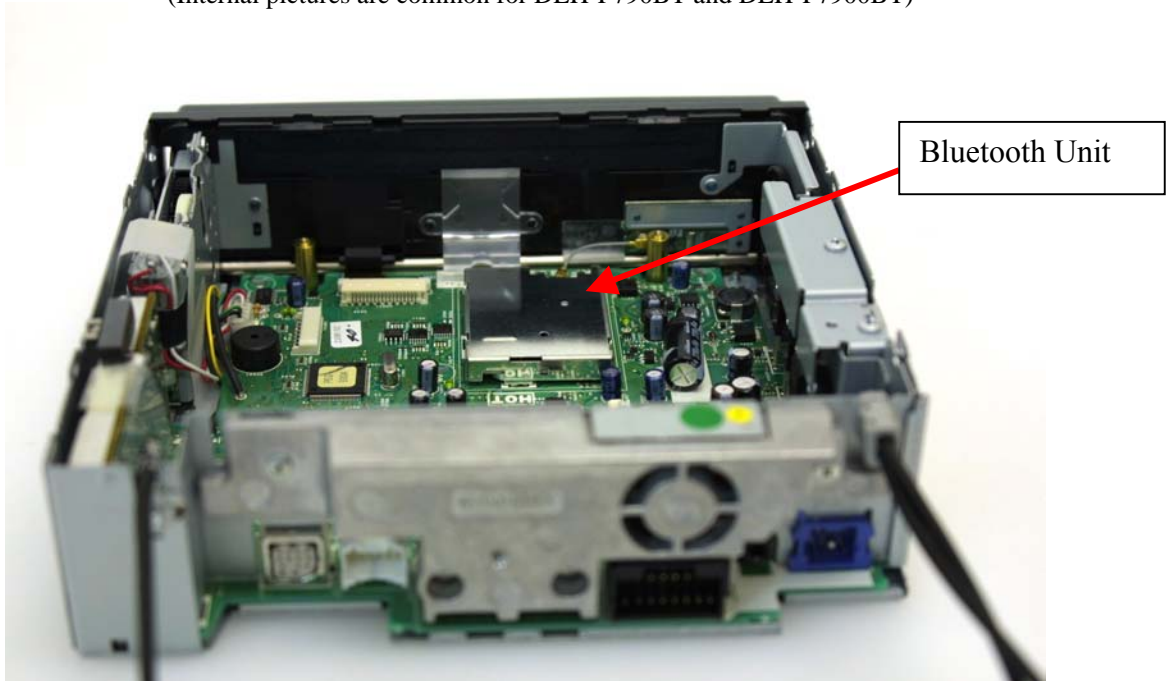
Internal View
