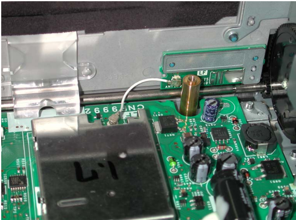
Connected with Antenna
