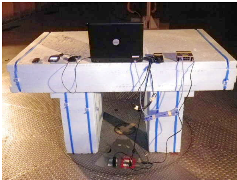
(Rear view)
