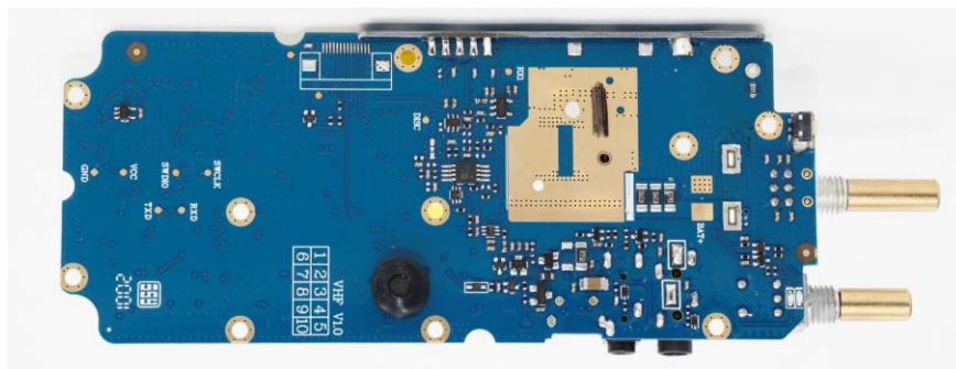
Internal Bottom-side View
