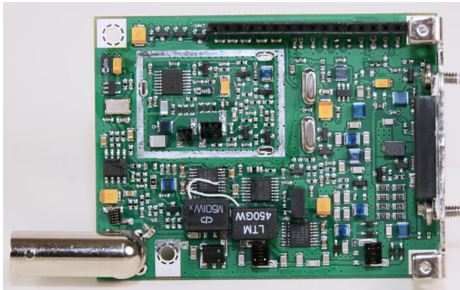
RF Board Top View w/o Shield
