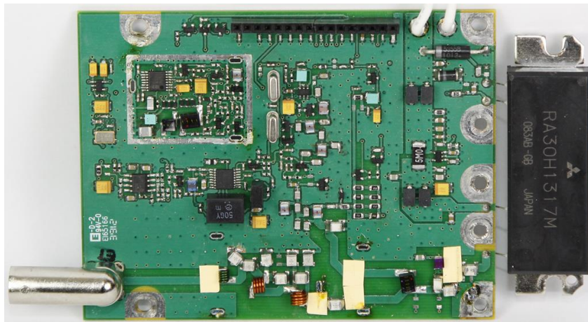
DTX-165 RF Board Top View w/o Shields
