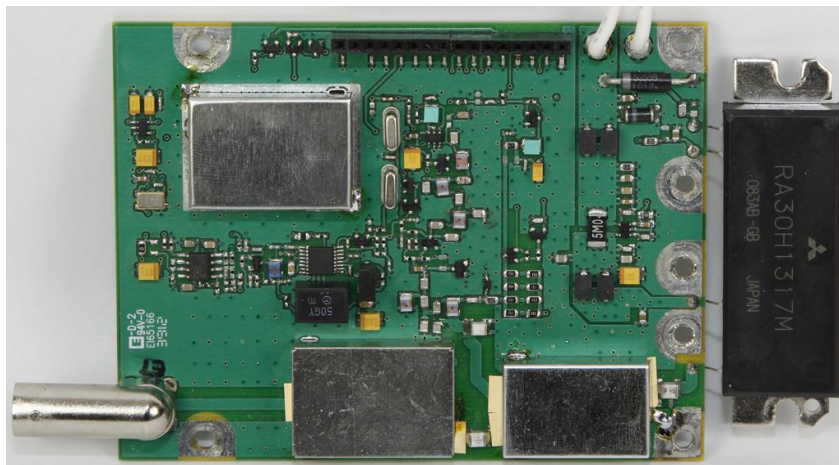
DTX-165 RF Board Top View w/ Shields
