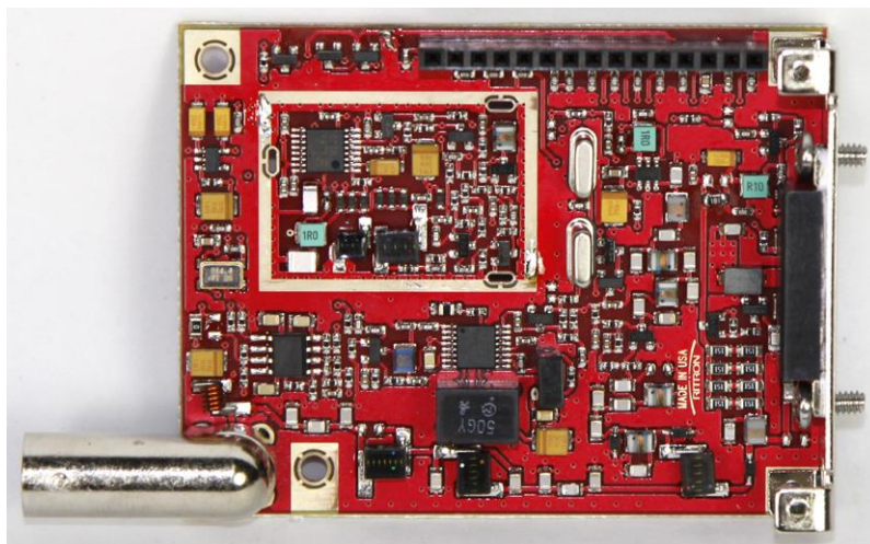
RF Board-Component Side, shields removed
