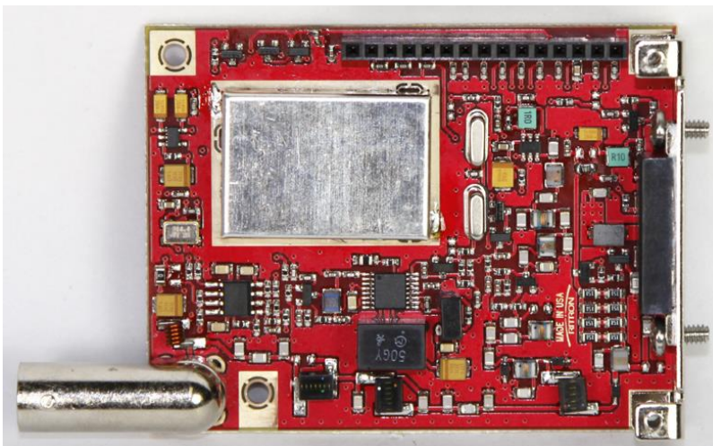
RF Board-Component side with shields
