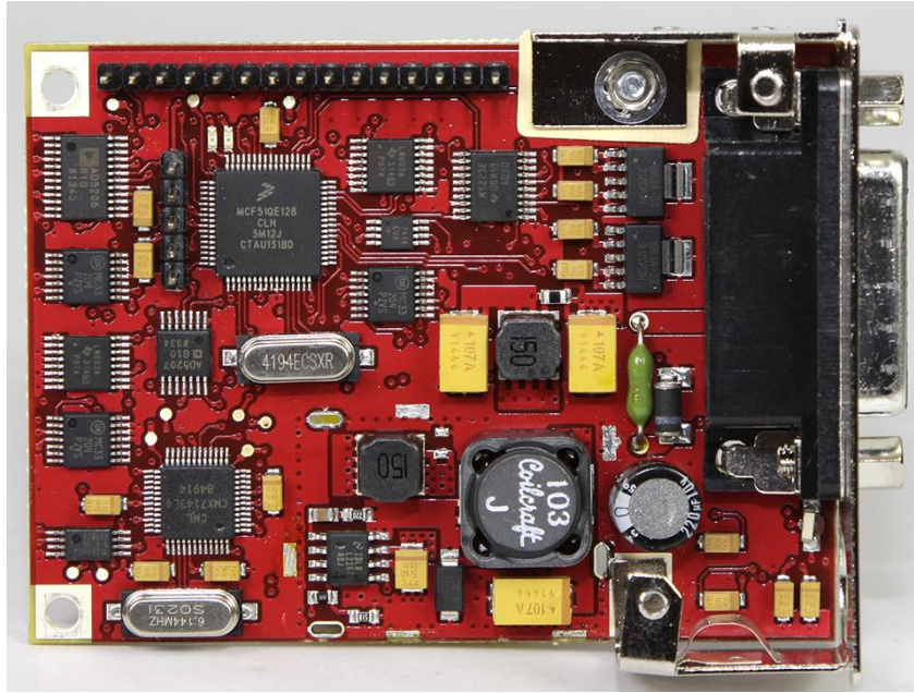
Modem Board-Component Side, shields removed
