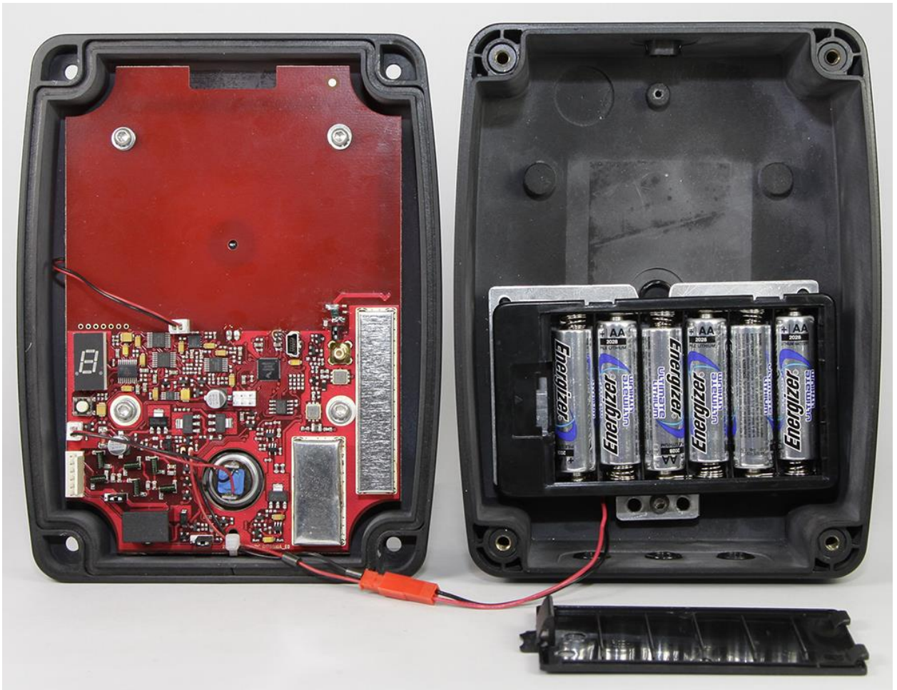
EXHIBIT: RQX-456 with 6 AA-cell batteries. Case open to show printed circuit board installation FCC ID: AIERIT38-456
