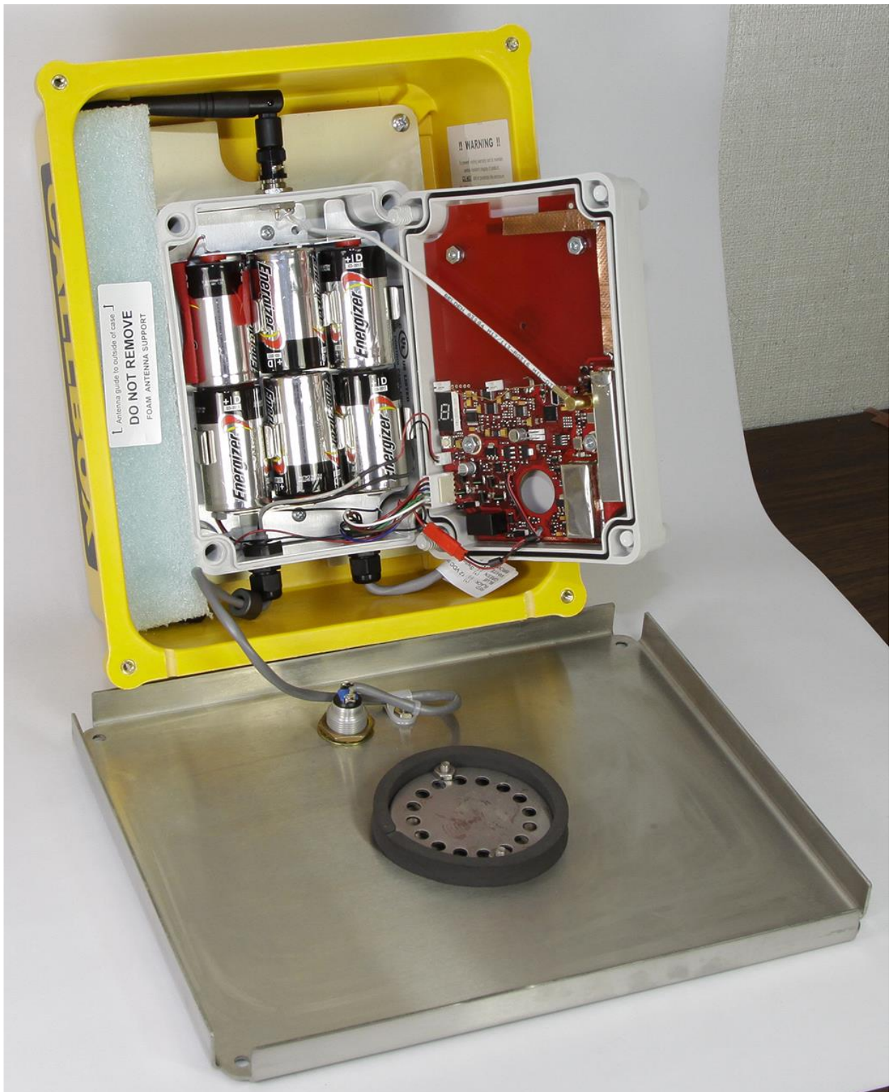
EXHIBIT: RQX-456-XT with 6 D-cell batteries. Case open to show printed circuit board installation FCC ID: AIERIT38-456
