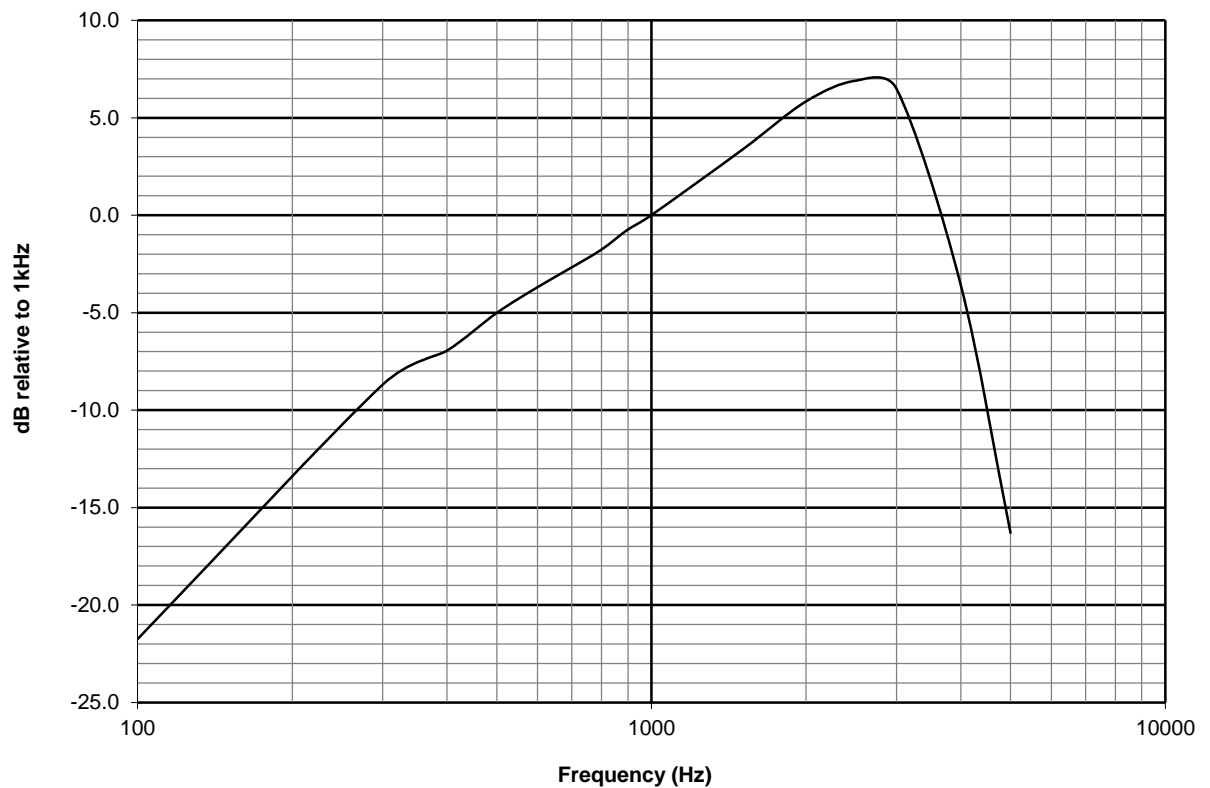
RQX-156 TX Audio Overall Response
