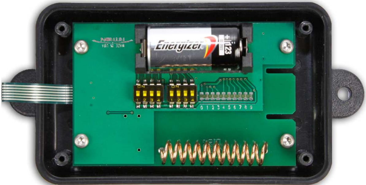
EXHIBIT: PCB installed in case back with battery installed FCC ID: AIERIT35-433
