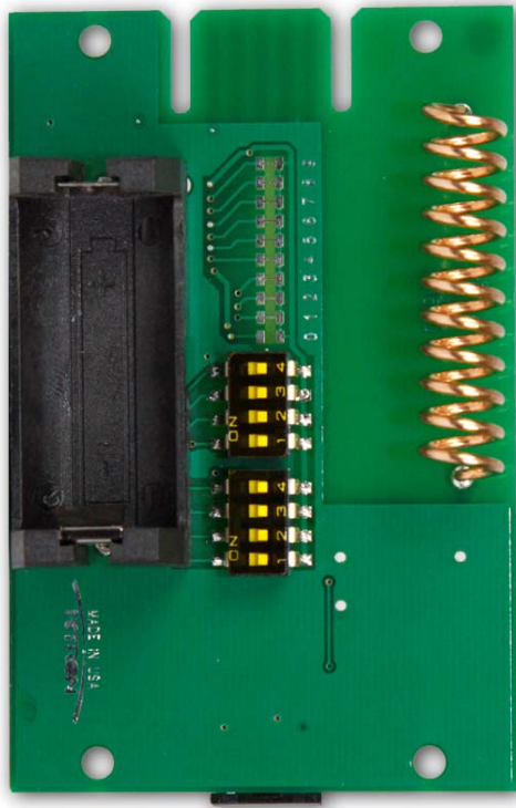
EXHIBIT: PCB topside FCC ID: AIERIT35-433
