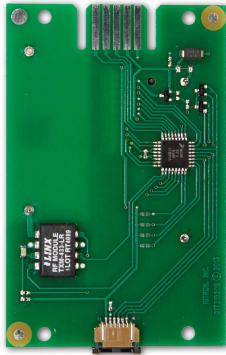
EXHIBIT: PCB bottom side FCC ID: AIERIT35-433
