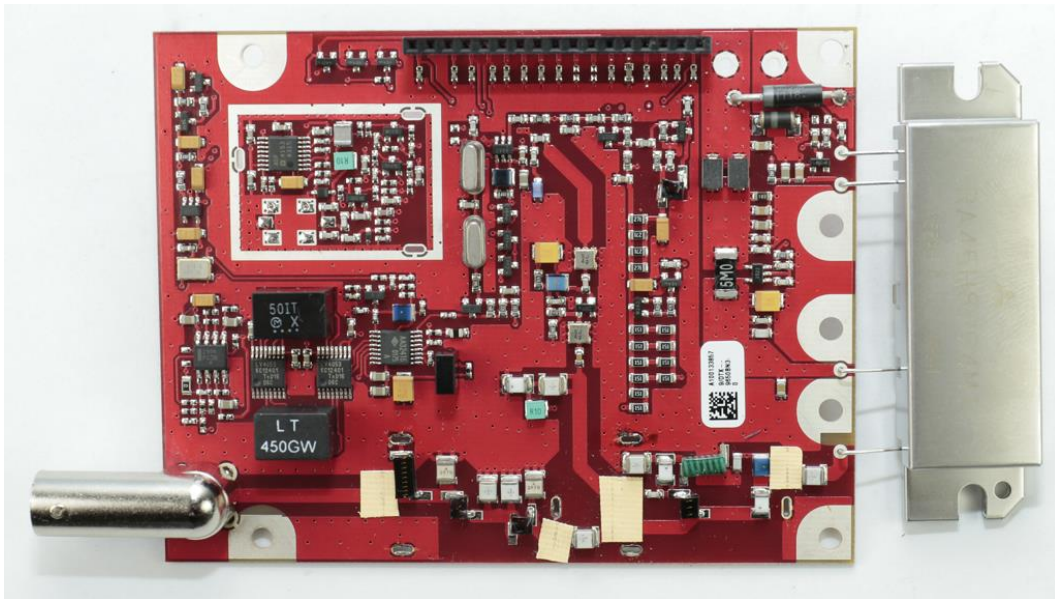
DTX-965 RF Board Top View w/o Shields
