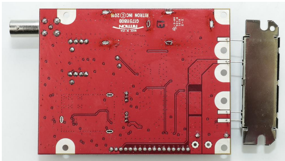
DTX-965 RF Board Bottom View
