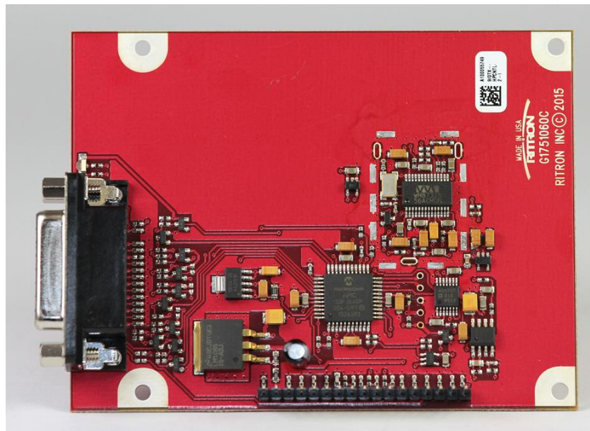
DTX-965 Control/Loader Board Top View w/o Shield
