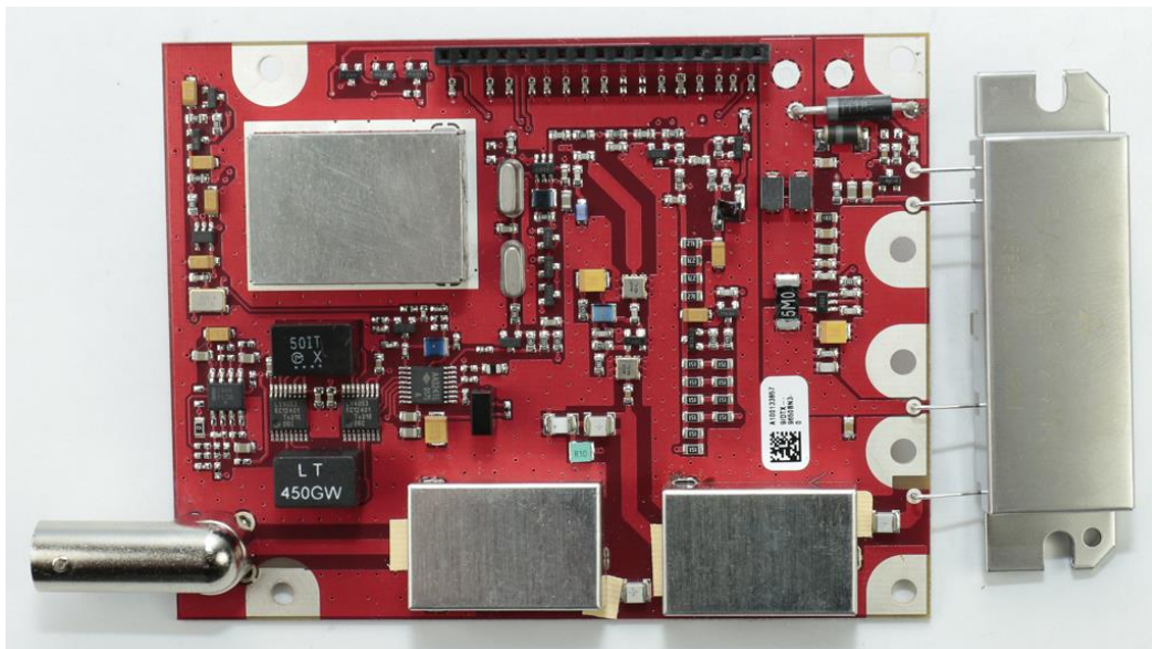
DTX-965 RF Board Top View w/ Shields
