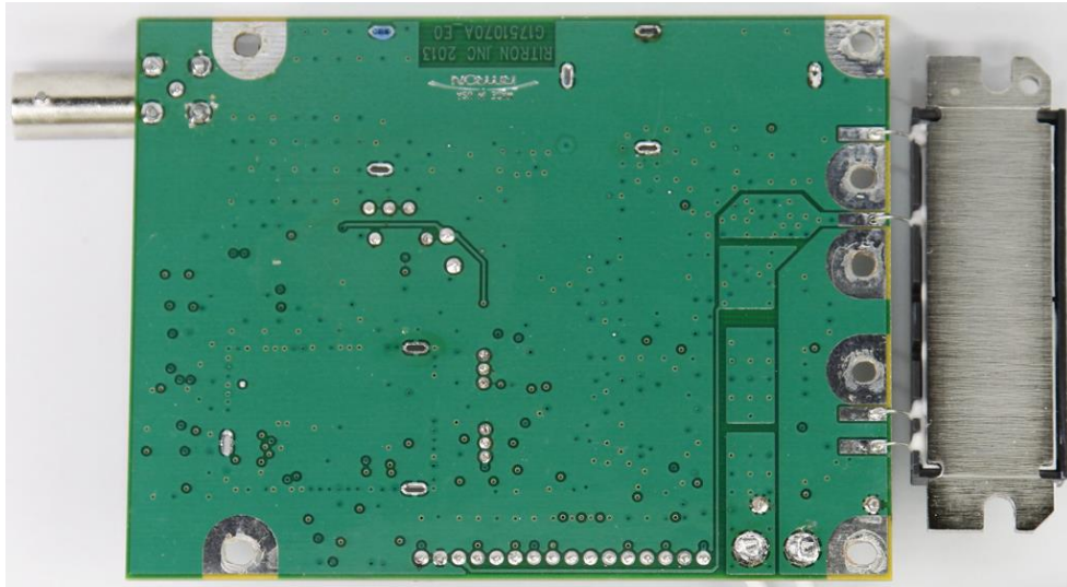
DTX-165-0BN30I-NX RF Board Bottom View
