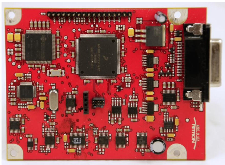
DTX-165-0BN30I-NX Control/Loader Board Top View
