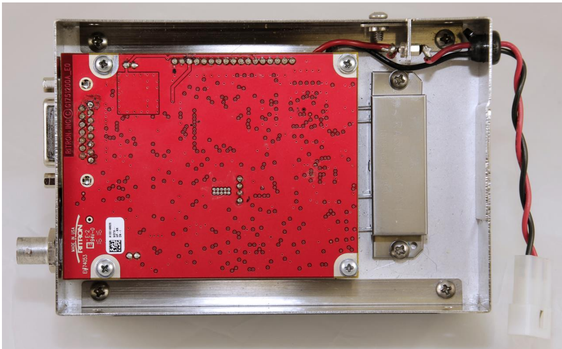
DTX-165-0BN30I-NX PCB/Heatsink Assembly w/ Enclosure Shield
