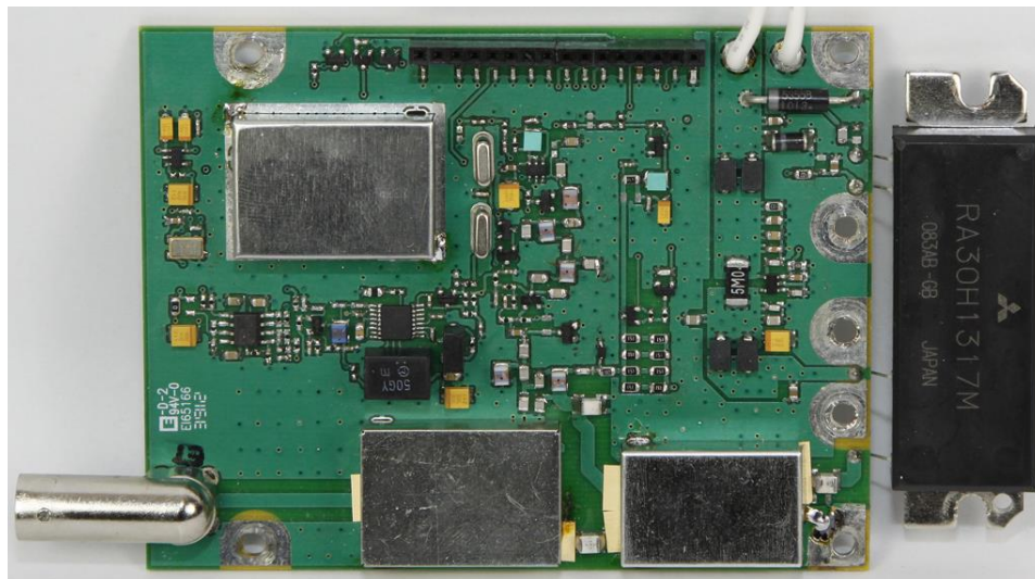
DTX-165-0BN30I-NX RF Board Top View w/ Shields
