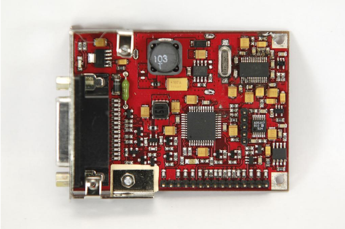
Control/Loader Board-Component Side, shields removed
