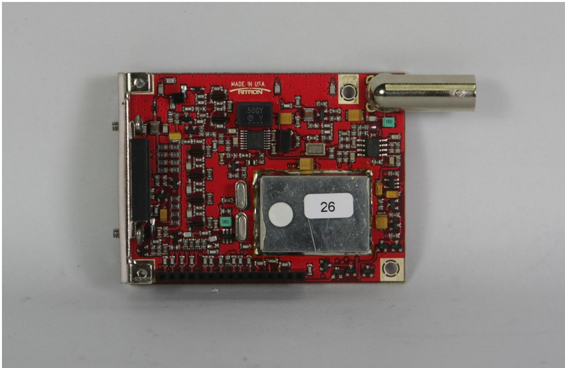
RF Board-Component side with shields
