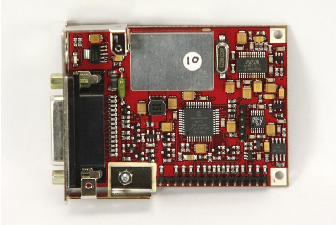
Control/Loader Board-Component Side without shields
