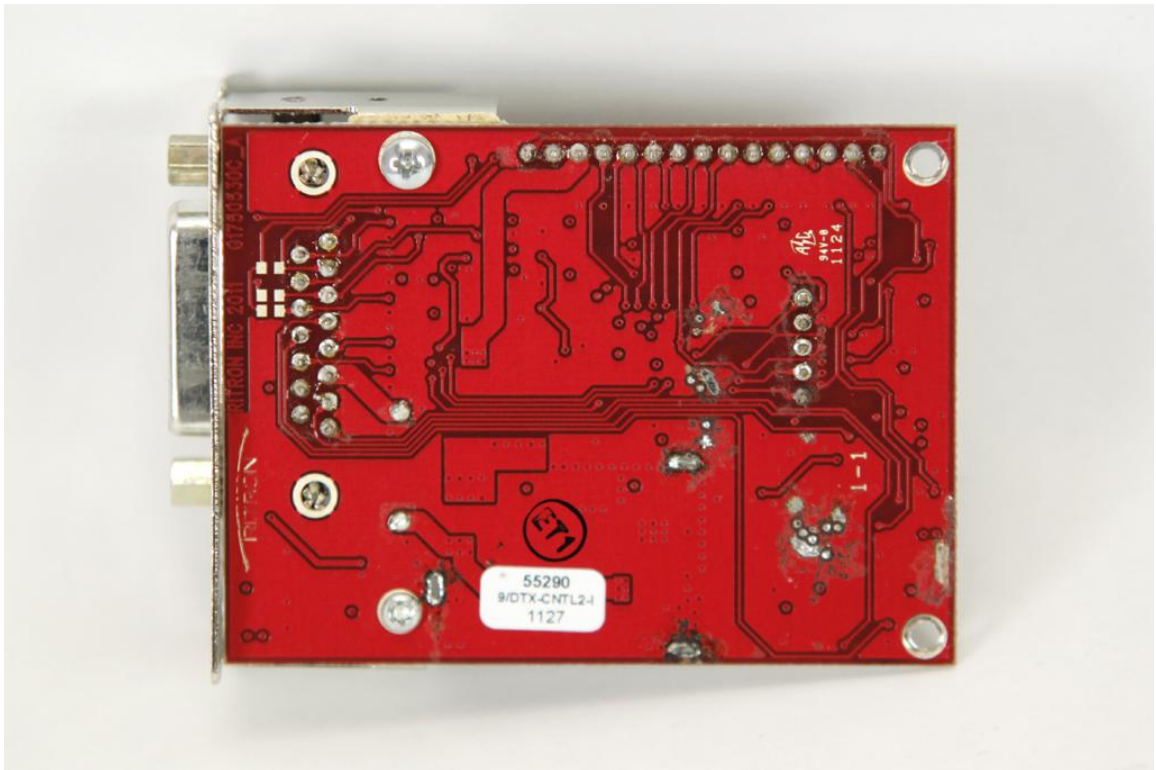
Control/Loader Board-Solder Side
