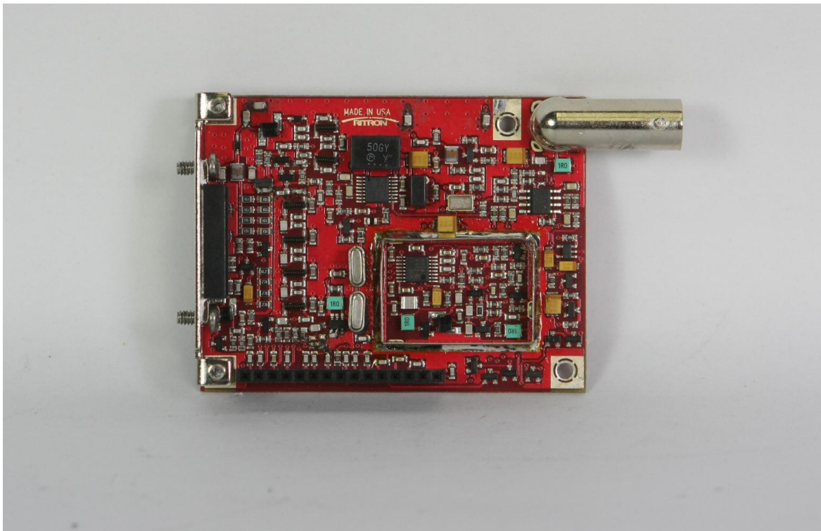
RF Board-Component Side, shields removed
