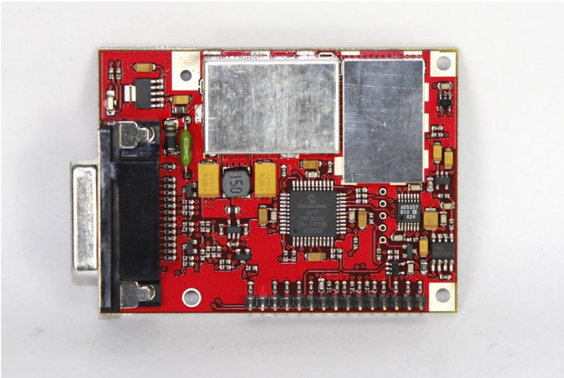
Control/Loader Board-Component Side with shields
