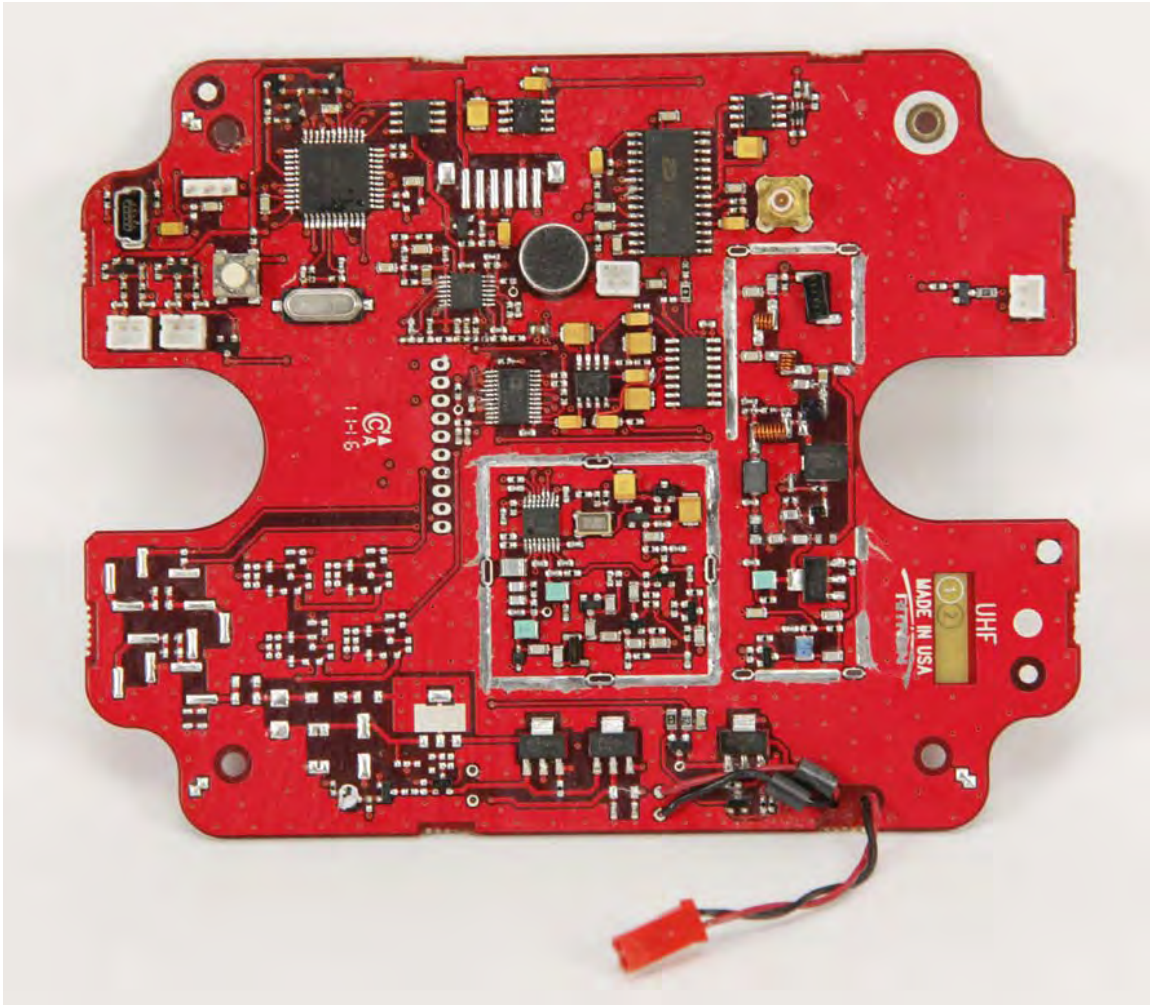
EXHIBIT: RQA-452 complete topside PCB assembly with shield removed FCC ID: AIERIT32-452
