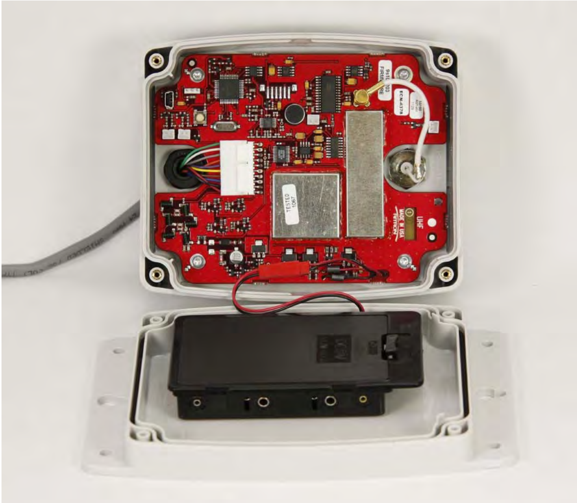
EXHIBIT: RQT-452 with case open to show printed circuit board installation FCC ID: AIERIT32-452
