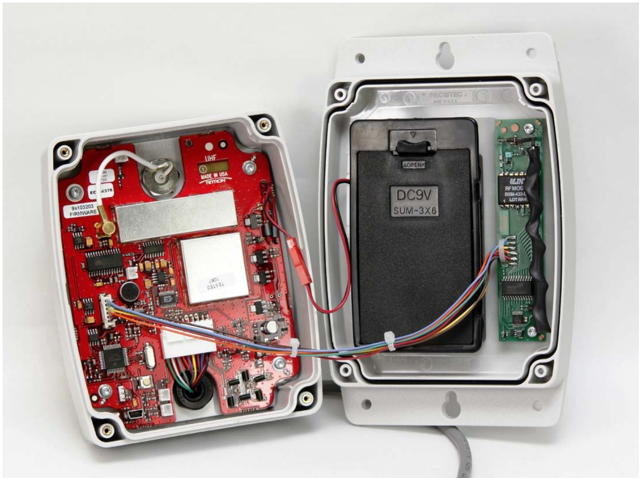
EXHIBIT: RQT-433-RCVR installed in Ritron Model RQT-451 with case open to show installation FCC ID: AIERIT32-433-RCVR
