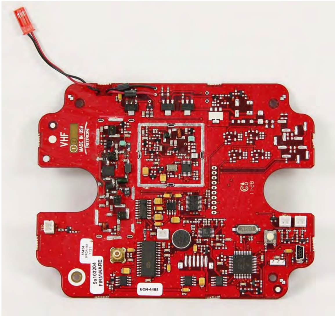
EXHIBIT: RQA-152M complete topside PCB assembly with shield removed FCC ID: AIERIT32-152M
