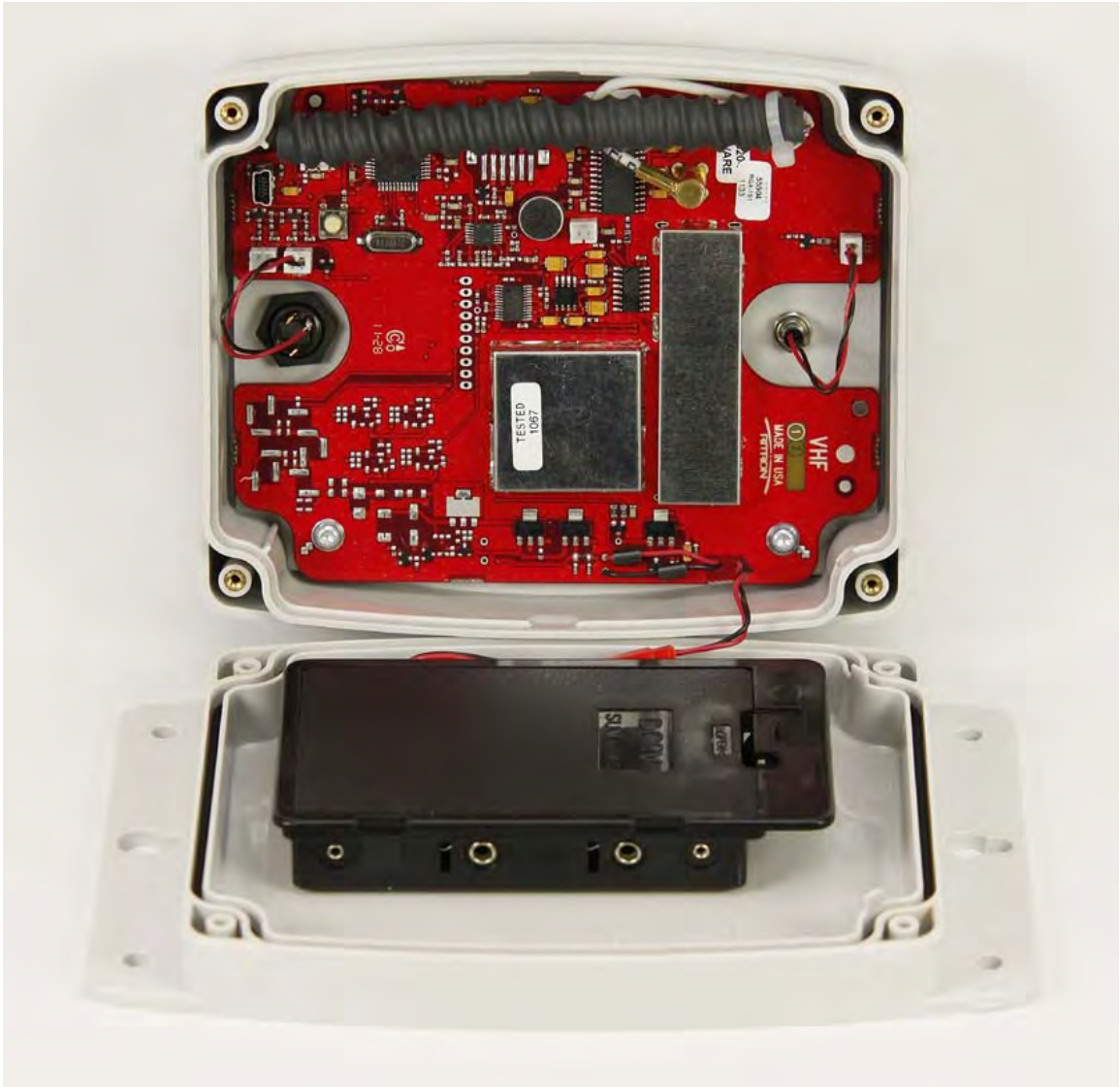
EXHIBIT: RQA-152M with case open to show printed circuit board installation FCC ID: AIERIT32-152M
