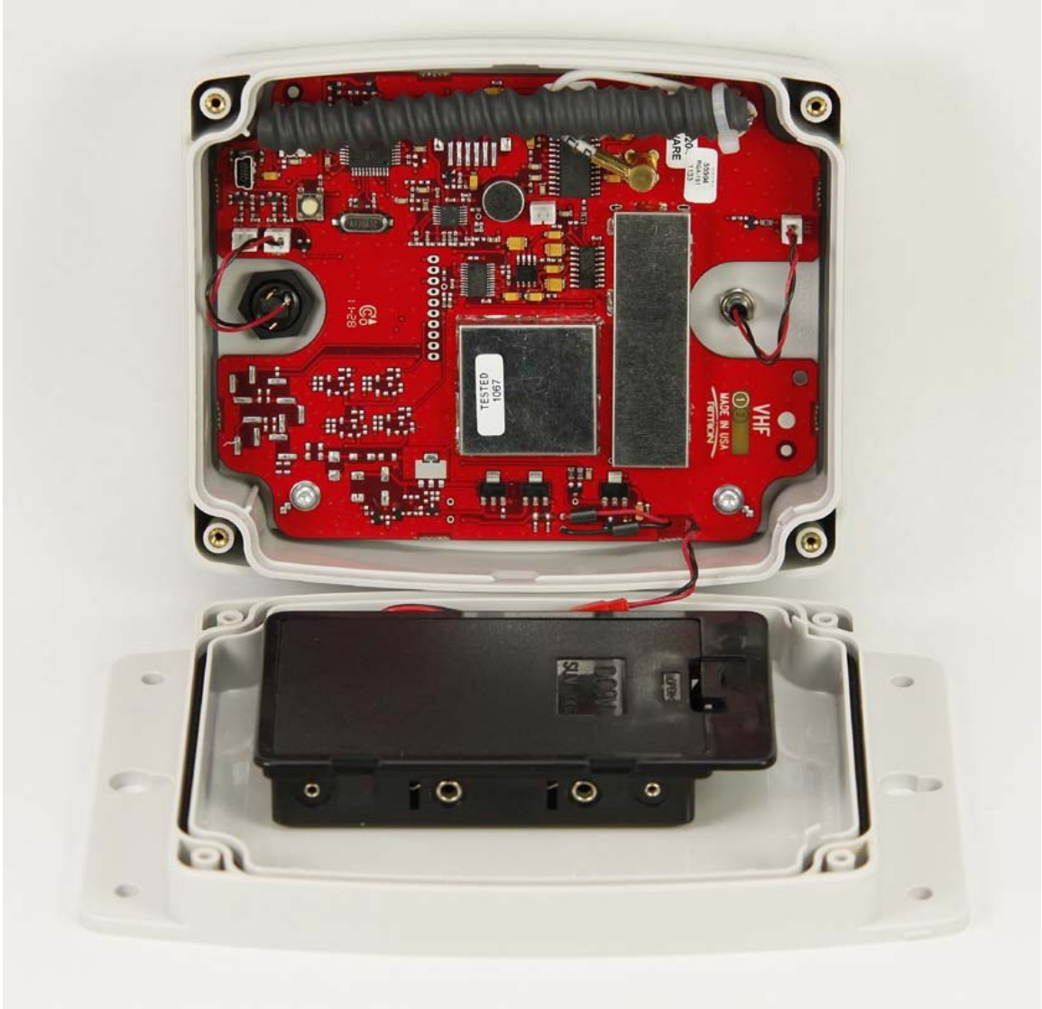
EXHIBIT: RQA-152 with case open to show printed circuit board installation FCC ID: AIERIT32-152
