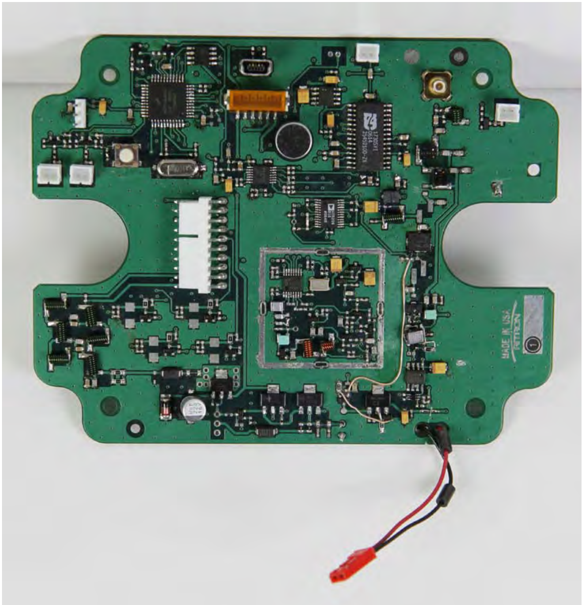
EXHIBIT: RQT-151M complete topside PCB assembly with shield removed FCC ID: AIERIT32-151M
