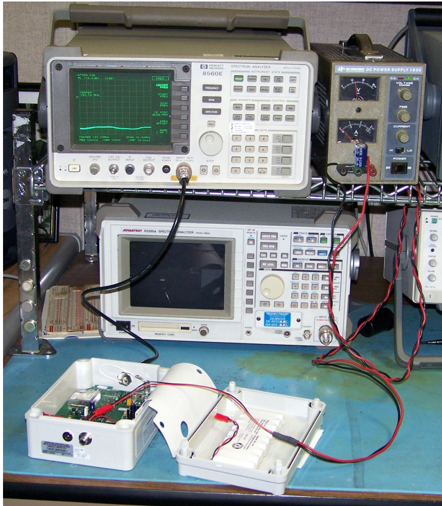
Test set-up for testing LM-V150 and LPA-V150 per FCC Part 15.111(a)
