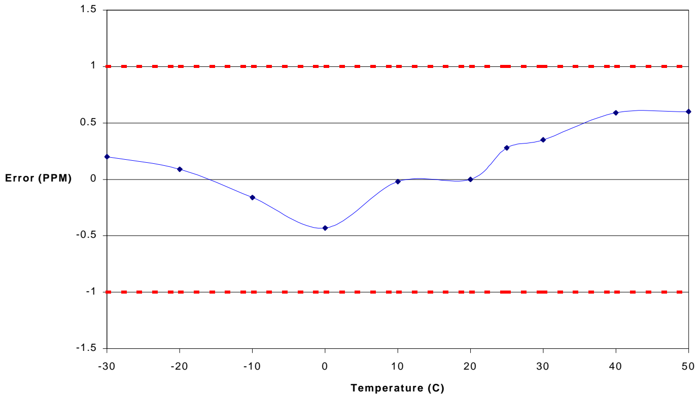
Frequency Error vs Temperature
