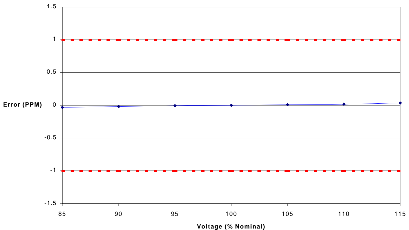
Frequency Error vs Supply Voltage
